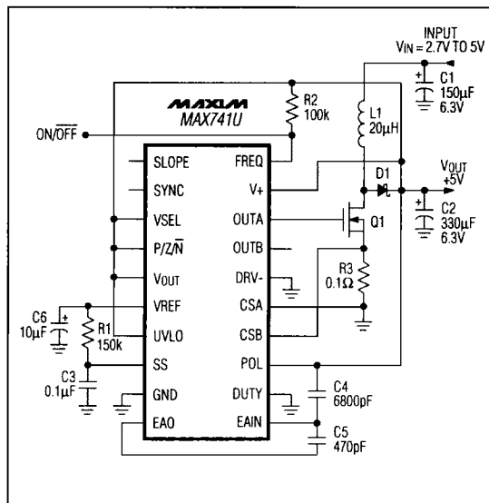
Figure 6. MAX741U EV Kit Schematic. This step-up converter supplies +5V at 1A from a +3V input.
