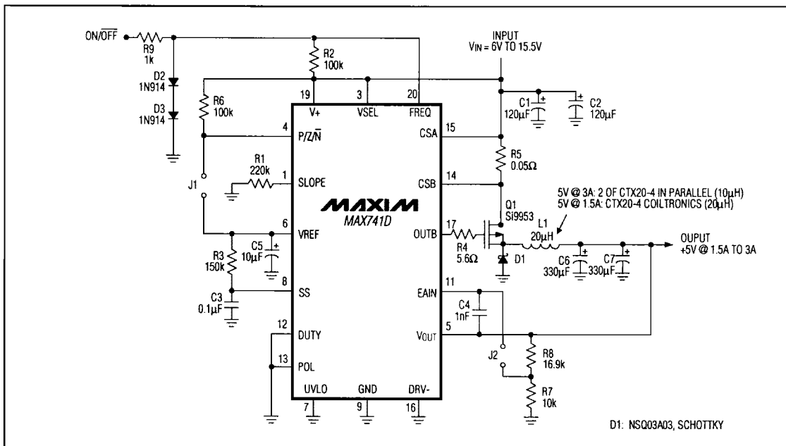
Figure 7. MAX741D EV Kit Schematic. +6V to +15.5V Input Step-Down Converter Supplies +5V at 1.5A or 3A.
