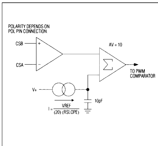
Figure 3. Current Amplifier and Slope Compensation Model
