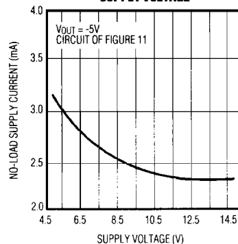
MAX741N INVERTING NO-LOAD SUPPLY CURRENT vs. SUPPLY VOLTAGE
