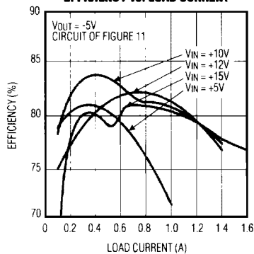
MAX741N INVERTING EFFICIENCY vs. LOAD CURRENT
