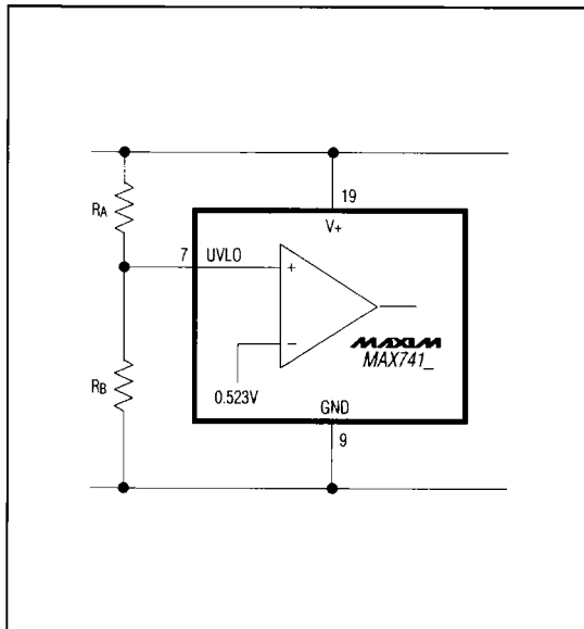
Figure 5. Undervoltage Lockout Comparator (Adjustable Mode)
