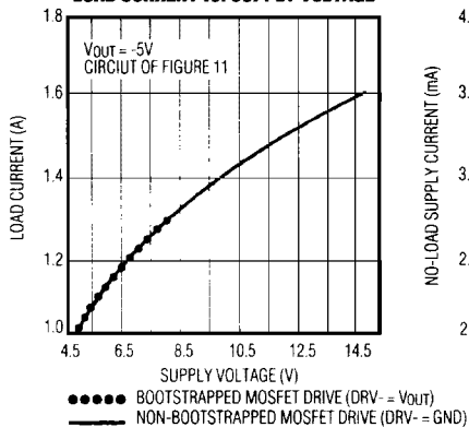
MAX741N INVERTING LOAD CURRENT vs. SUPPLY VOLTAGE
