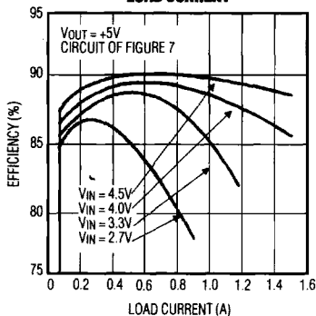
MAX741U STEP-UP EFFICIENCY vs. LOAD CURRENT
