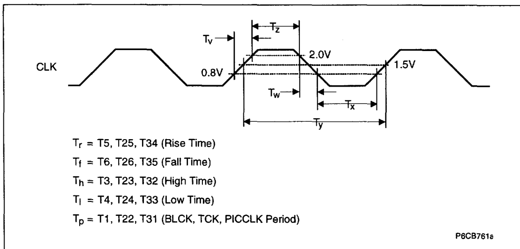
Figure 8. Valid Delay Timings
