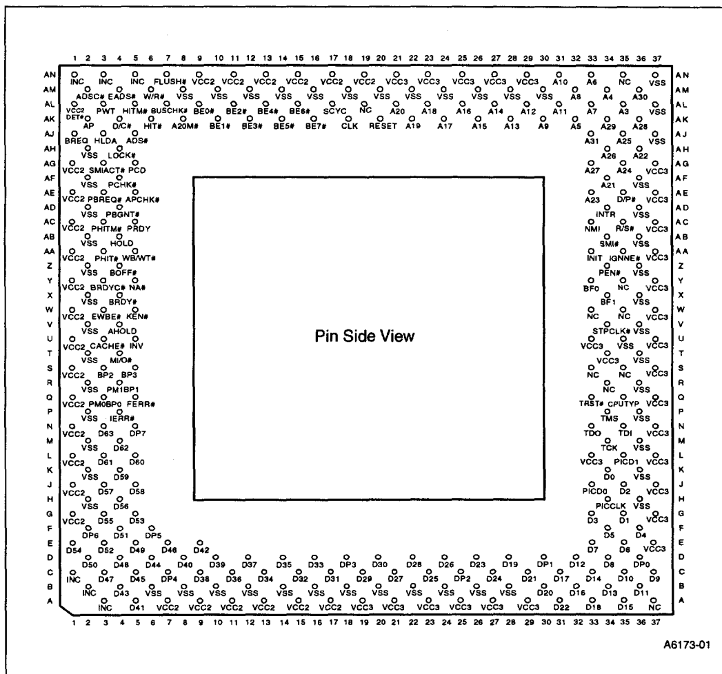
Figure 3. Pentium® Processor with MMX™ Technology PPGA Package Pinout - Bottom Side View
