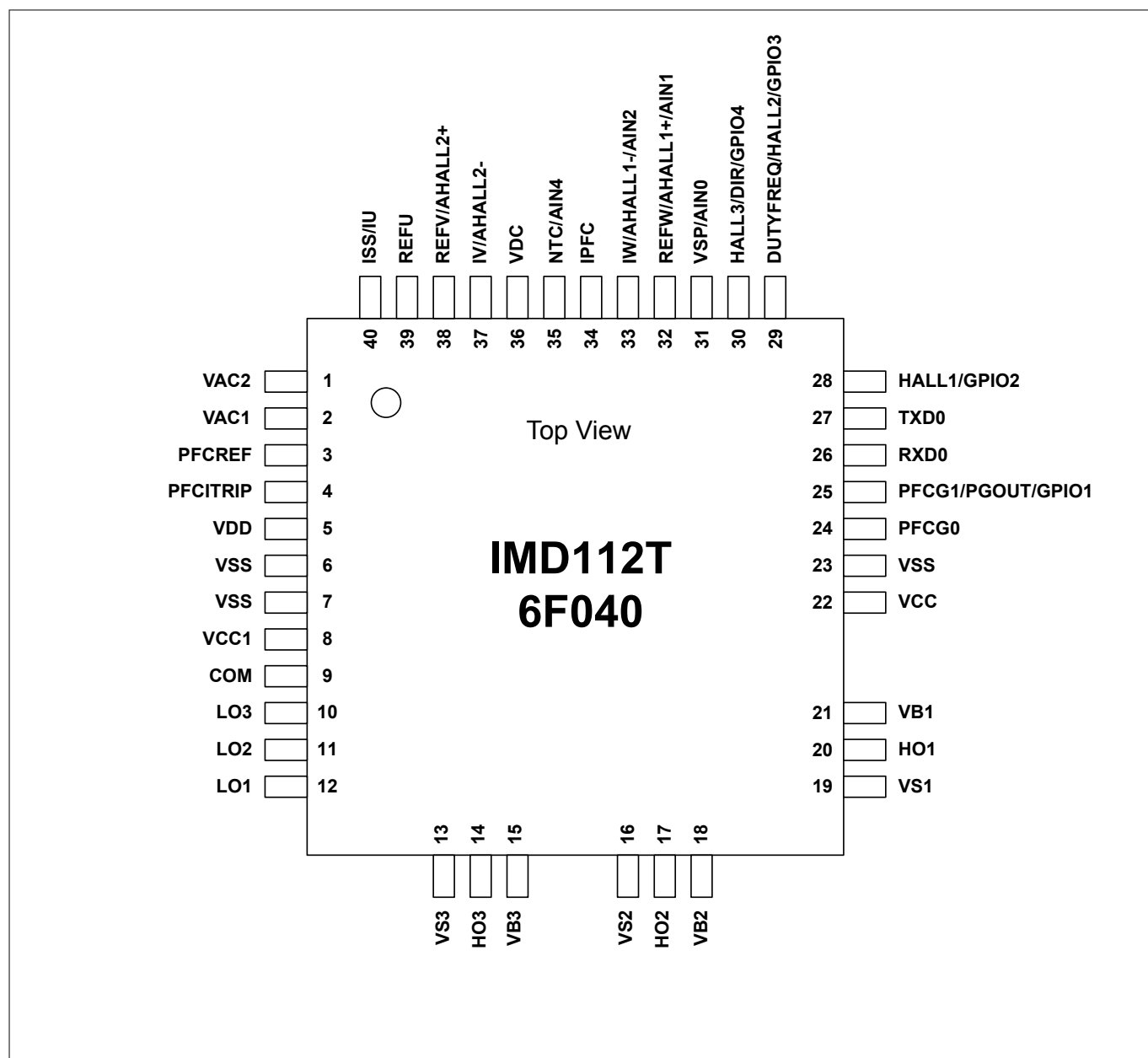
Figure 5 IMD112T-6F040
