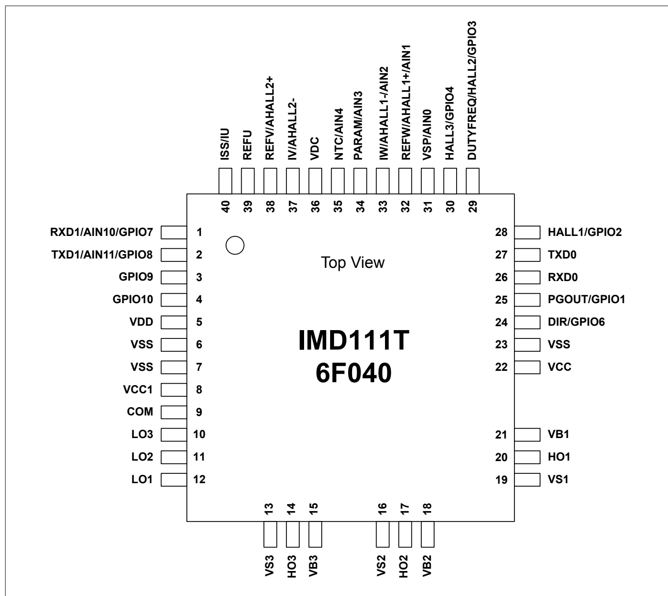
Figure 4 IMD111T-6F040
