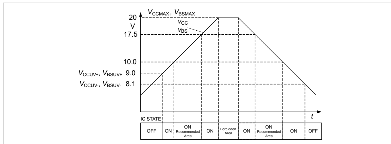
Figure 13 Operating Areas
