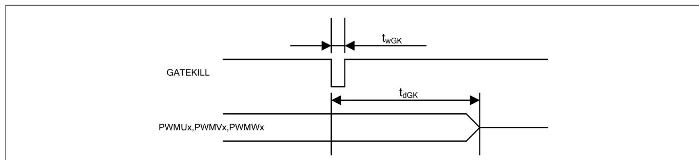
Figure 14 Fault timing
