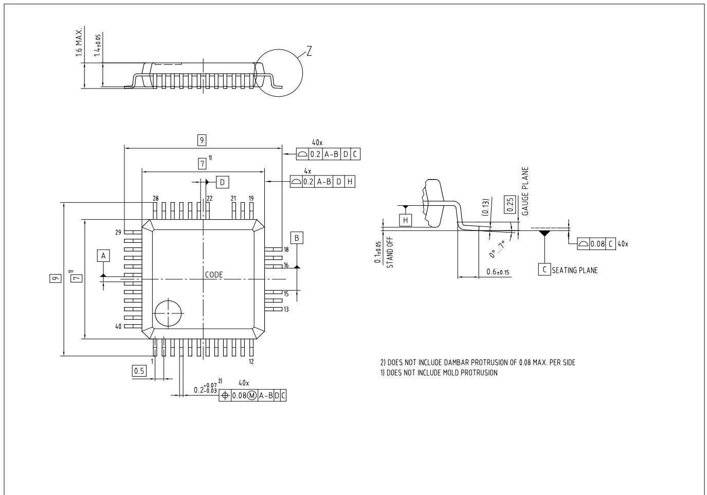
Figure 16 PG-LQFP-40-1
