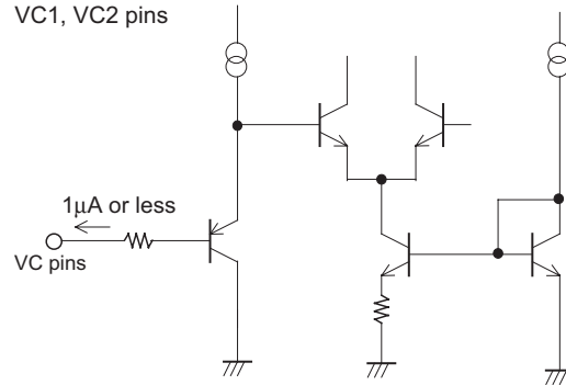
VC1, VC2 pins
