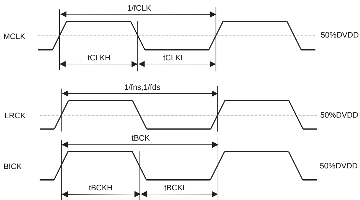
Clock Timing
