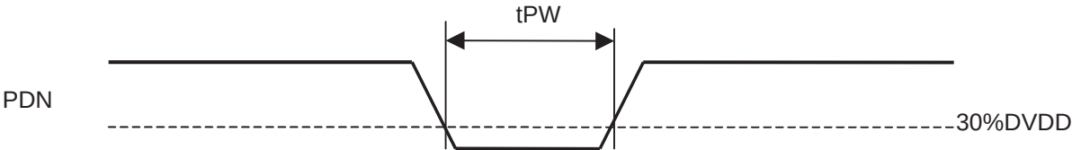
Power-down Timing
