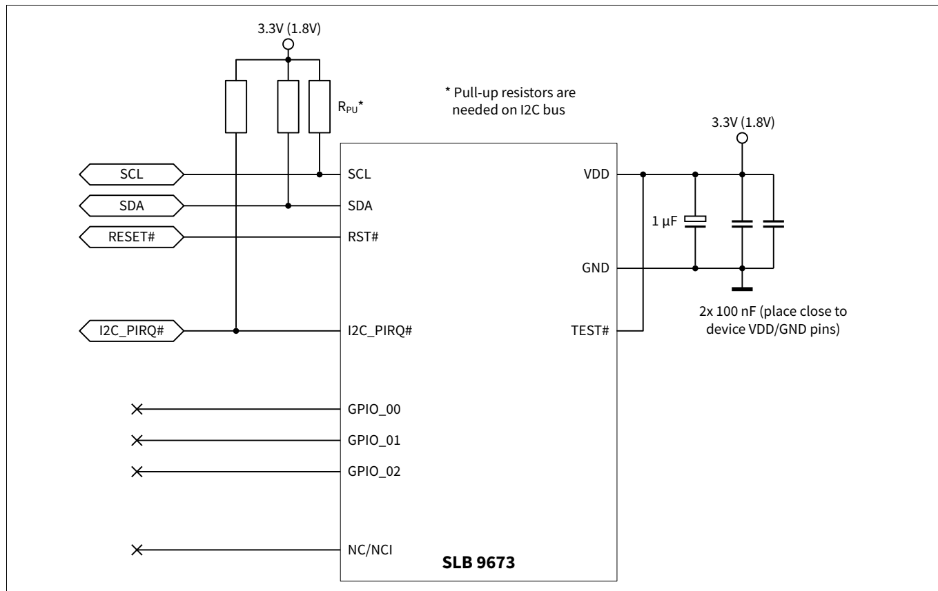
Figure 2 Typical schematic
