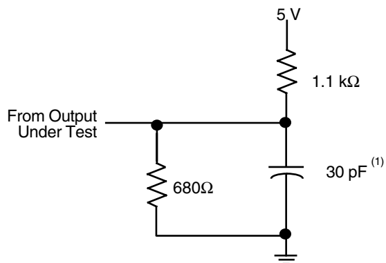
LOAD CIRCUIT
