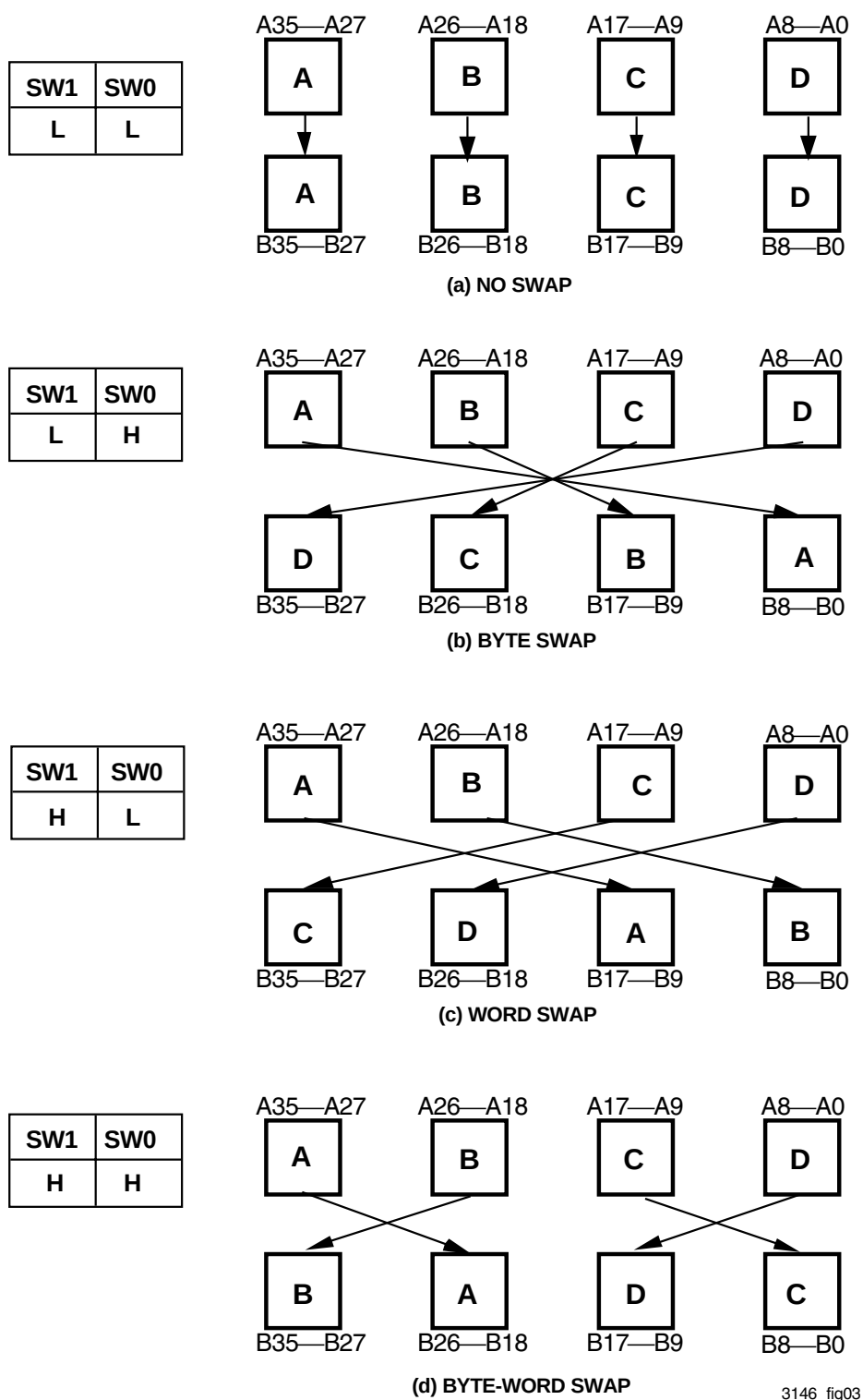
Figure 4. Byte Swapping (Long Word Size Example)
