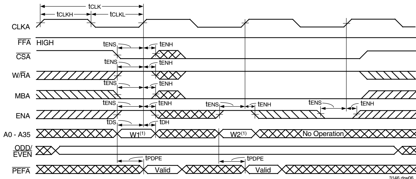
Figure 6. Port-A Write Cycle Timing for FIFO1
