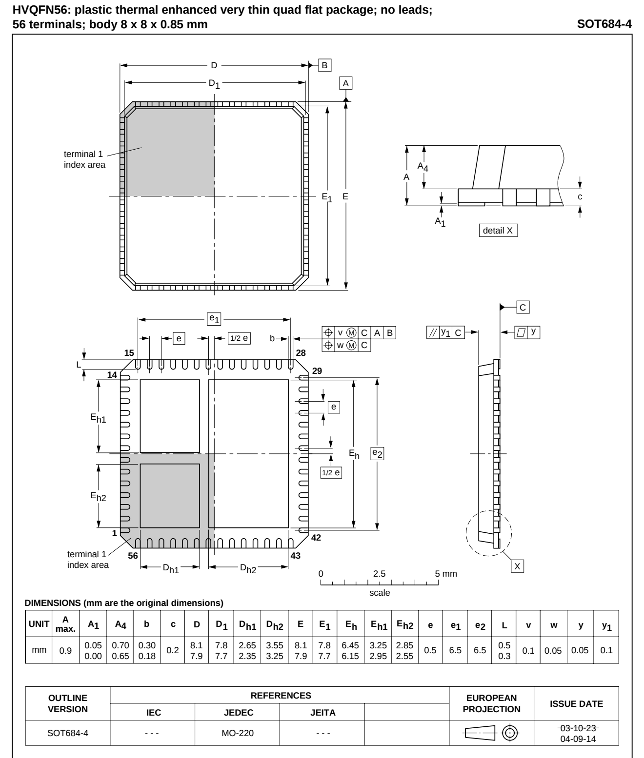
Fig 16. Package outline SOT684-4 (HVQFN56)
