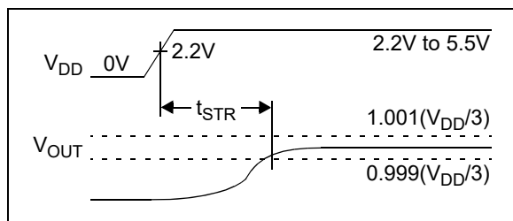
FIGURE 1-1: Amplifier Start-up.
