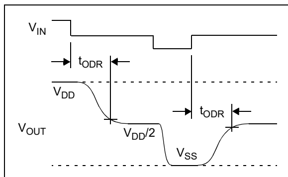
FIGURE 1-3: Output Overdrive Recovery.
