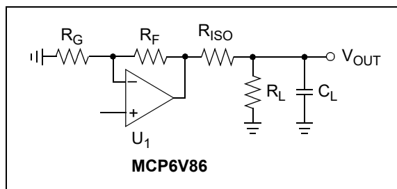
FIGURE 4-9: Output Load.
