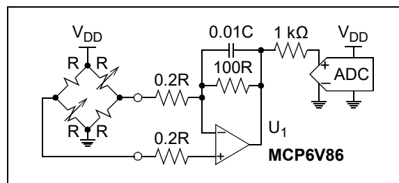
FIGURE 4-11: Simple Design.
