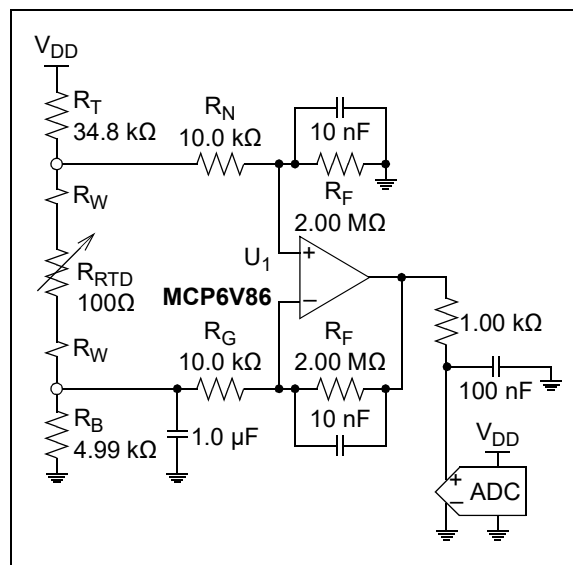
FIGURE 4-12: RTD Sensor.
