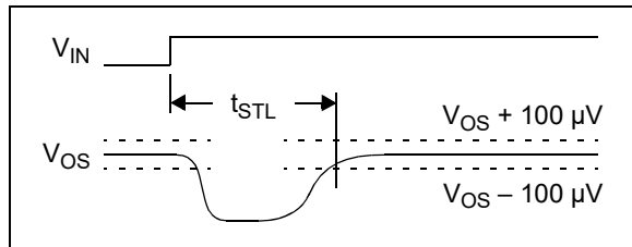
FIGURE 1-2: Offset Correction Settling Time.
