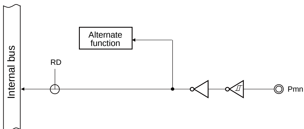
Figure 2-3. Pin Block Diagram for Pin Type 2-1-2
