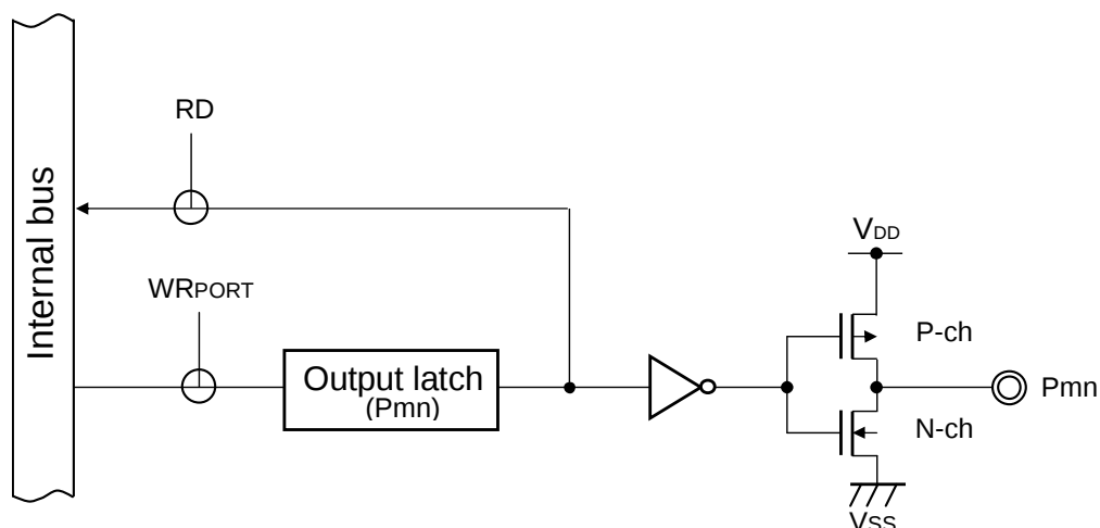
Figure 2-1. Pin Block Diagram for Pin Type 1-1-1
