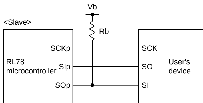
CSI mode connection diagram (during communication between devices at different potential)
