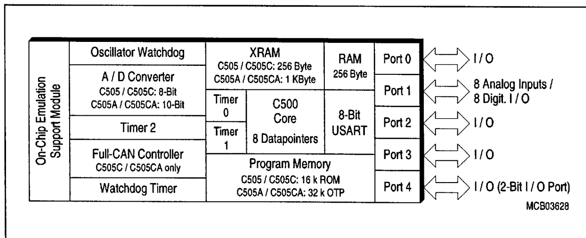
Figure 1 C505 Functional Units
