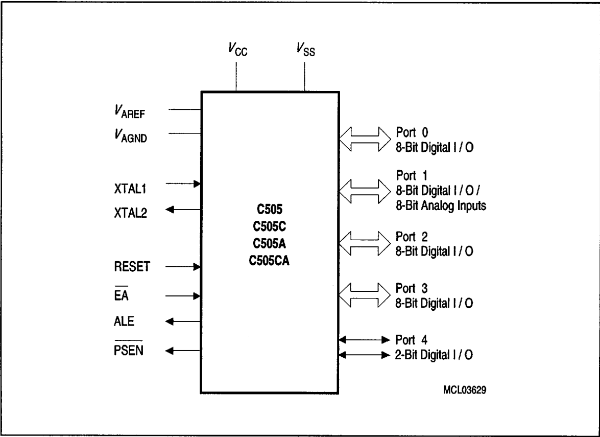
Figure 2 Logic Symbol
