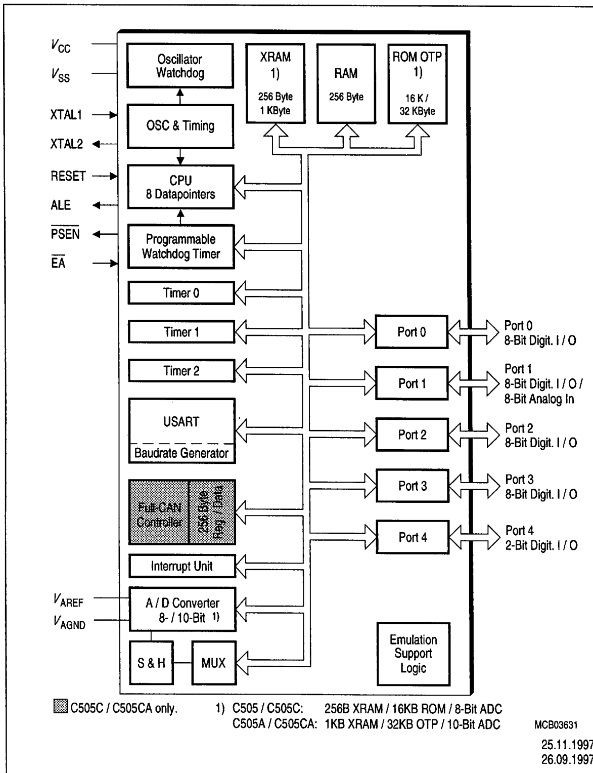
Figure 4 Block Diagram of the C505/C505C/C505A/C505CA
