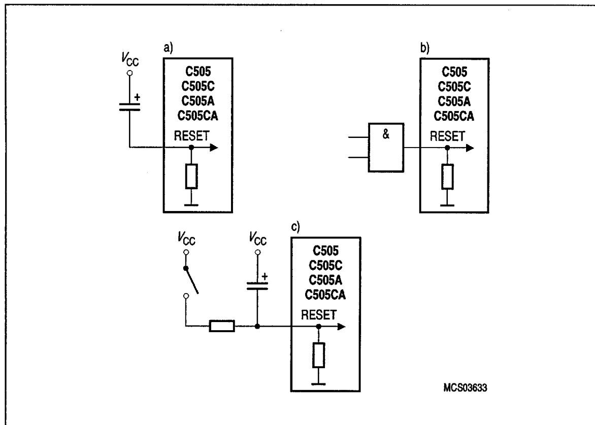
Figure 6 Reset Circuitries
