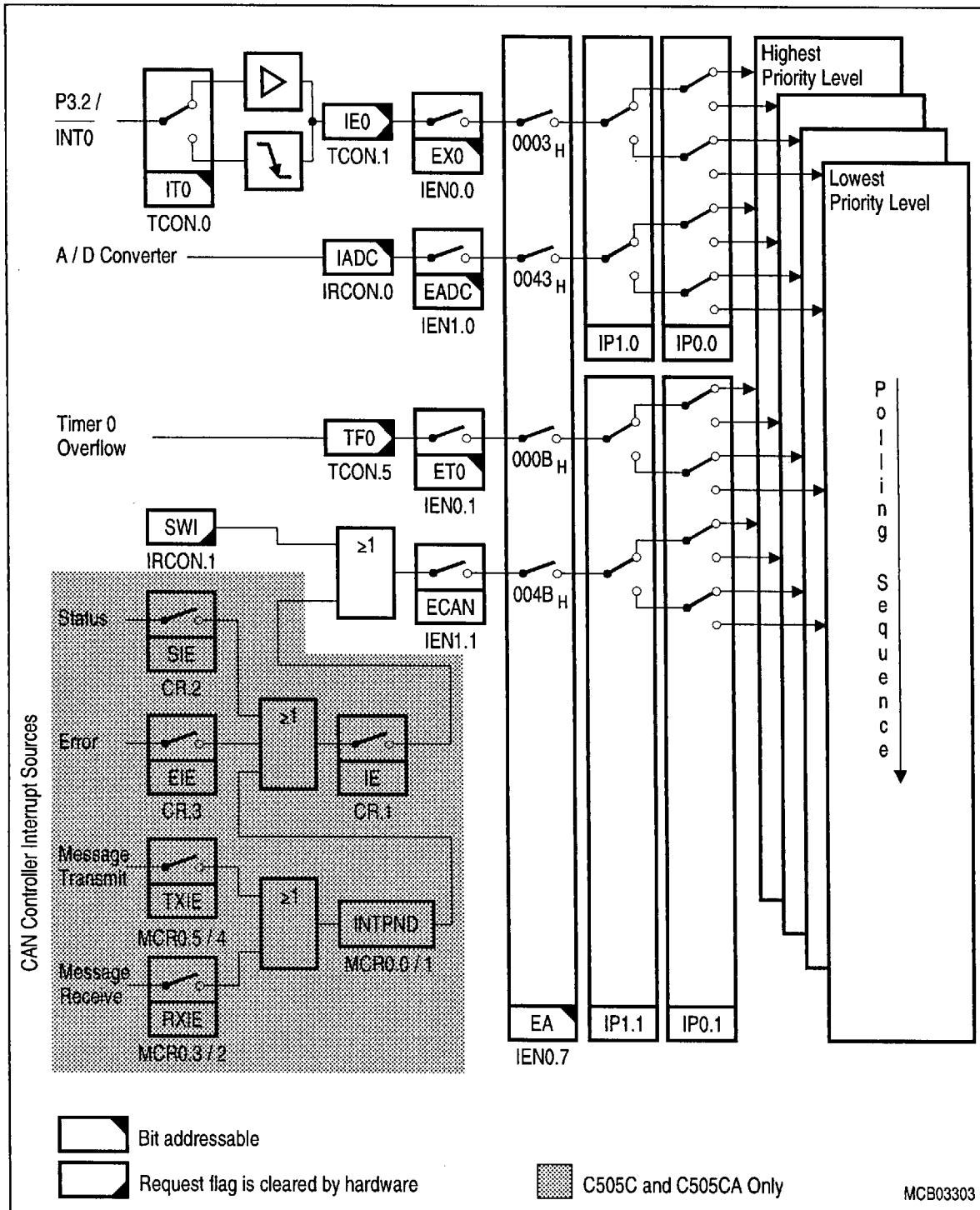
Figure 21 Interrupt Structure, Overview Part 1
