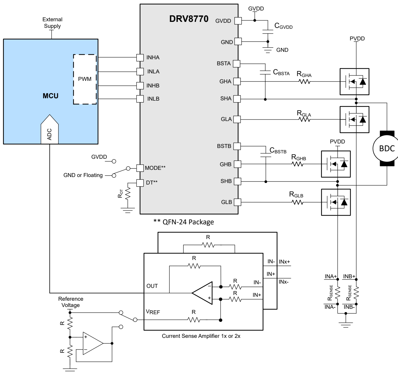
Figure 8-1. Application Schematic
