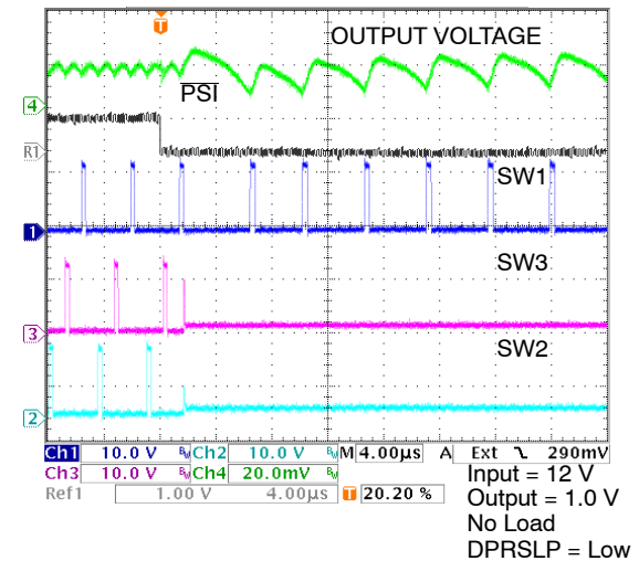
Figure 17. PSI Transition
