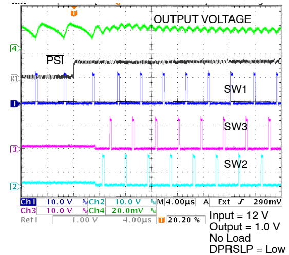
Figure 16. PSI Transition
