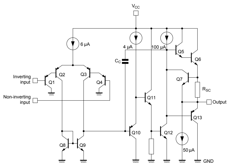
Figure 1. Schematic diagram (1/2 LM2904AH)
