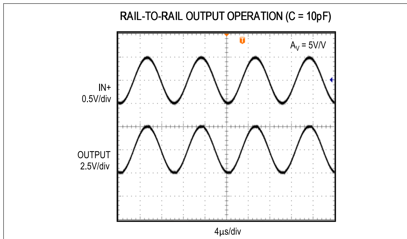
Figure 3. Rail-to-Rail Output Operation with 10k \Omega and A_V = 5V/V
