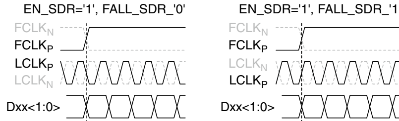
Figure 9. SDR interface modes
