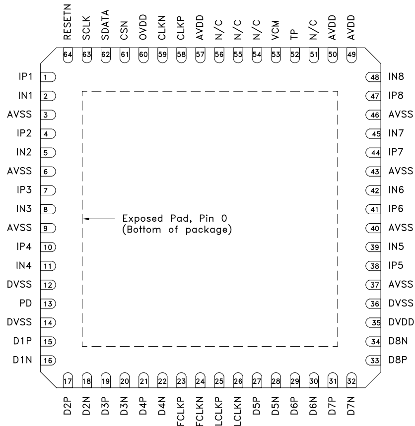
Figure 2. Package Diagram
