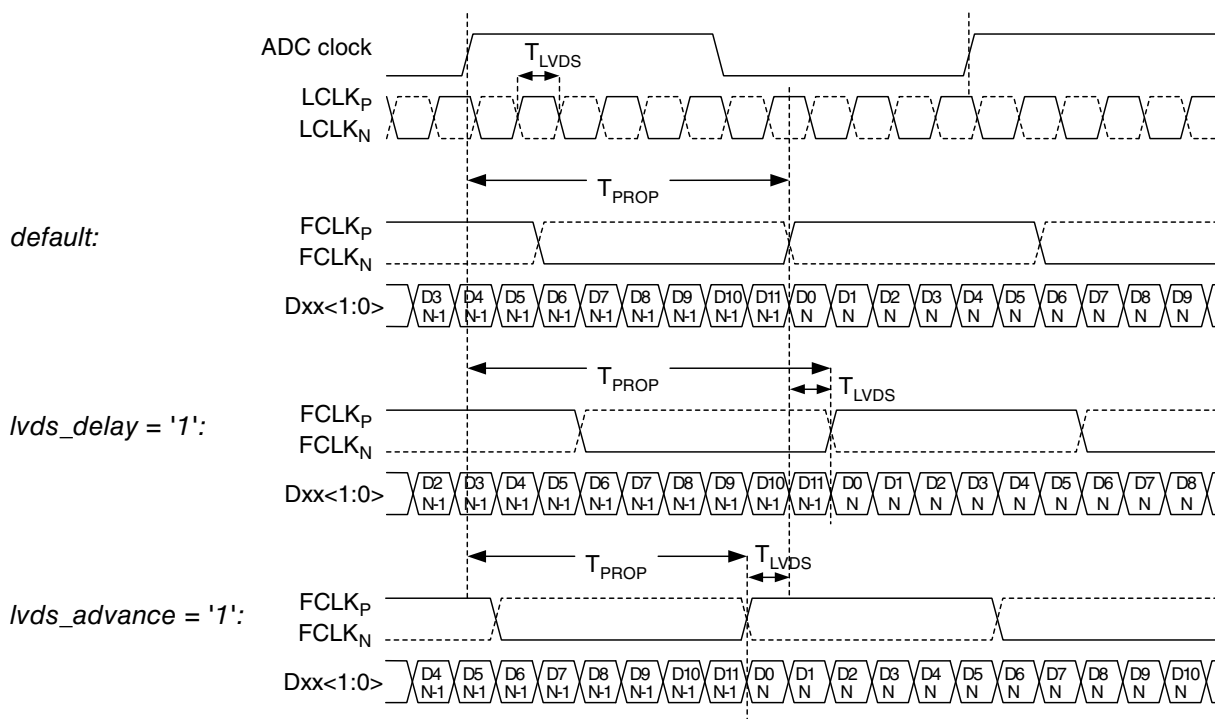
Figure 10. LVDS output timing adjustment
