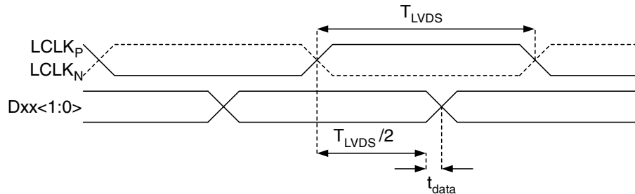
Figure 6. LVDS timing 12 bit output, SDR mode
