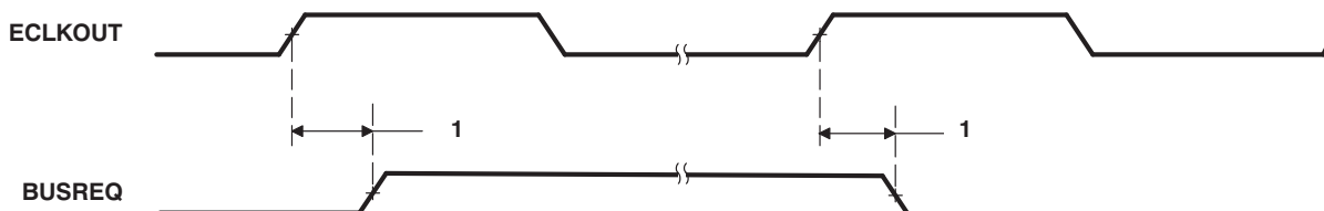
Figure 11-24. BUSREQ
