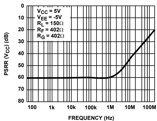
FIGURE 11. PSRR +5V
