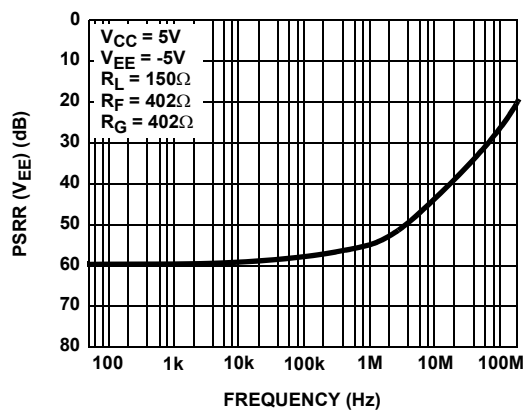
FIGURE 12. PSRR -5V
