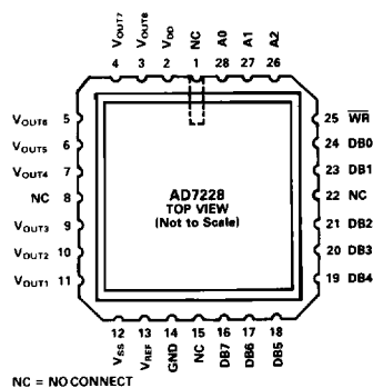
E Package (LCC)
