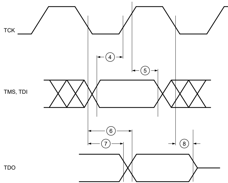
Figure 63. JTAG Test Access Port Timing
