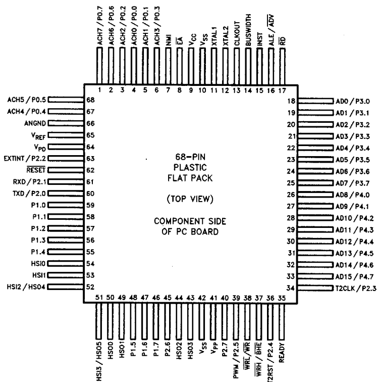
Figure 4. Package Diagrams
