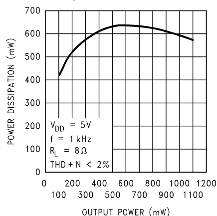
Power Dissipation vs Output Power, 5V, 8 \Omega
