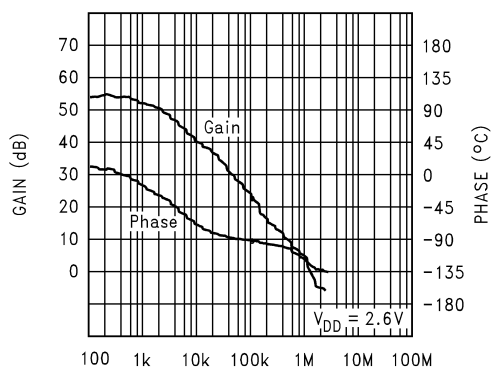
Open Loop Frequency Response, 2.6V
