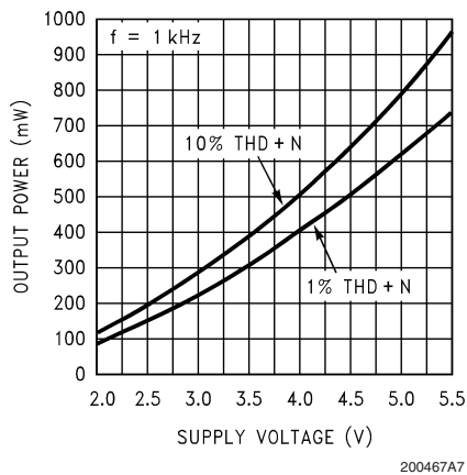
Output Power vs Supply Voltage, 16Ω
