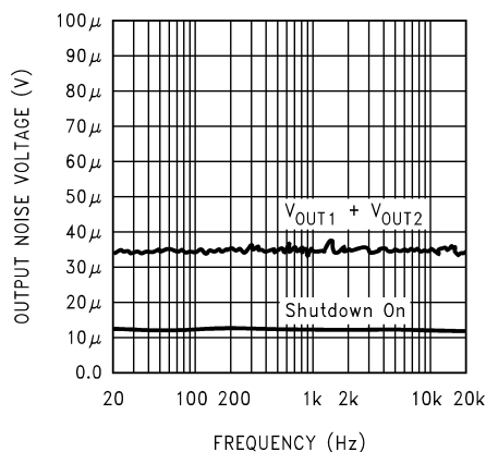
Noise Floor, 5V, 8 \Omega 80kHz Bandwidth, Input to GND
