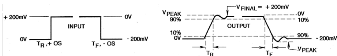
OVERSHOOT, RISE AND FALL TIME WAVEFORMS
