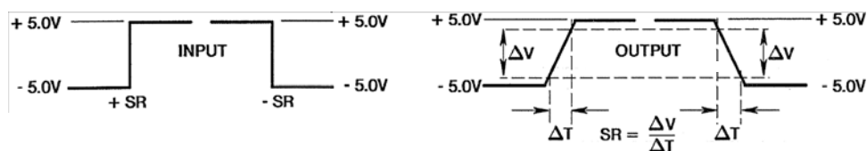
SLEW RATE WAVEFORMS
