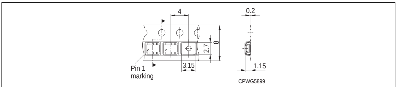
Figure 4 Tape loading
