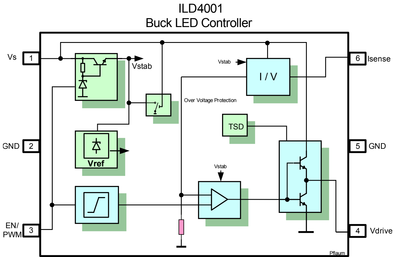
Figure 1 Block diagram
