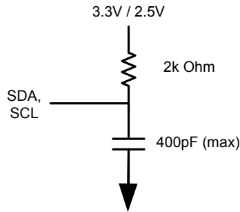
Figure 6: AC Output Test Load (I²C)
