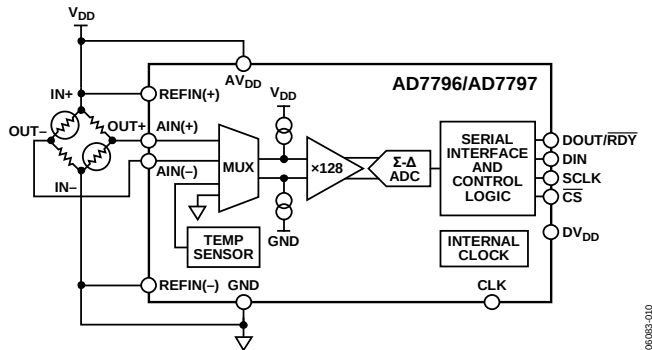
Figure 10. Basic Connection Diagram
