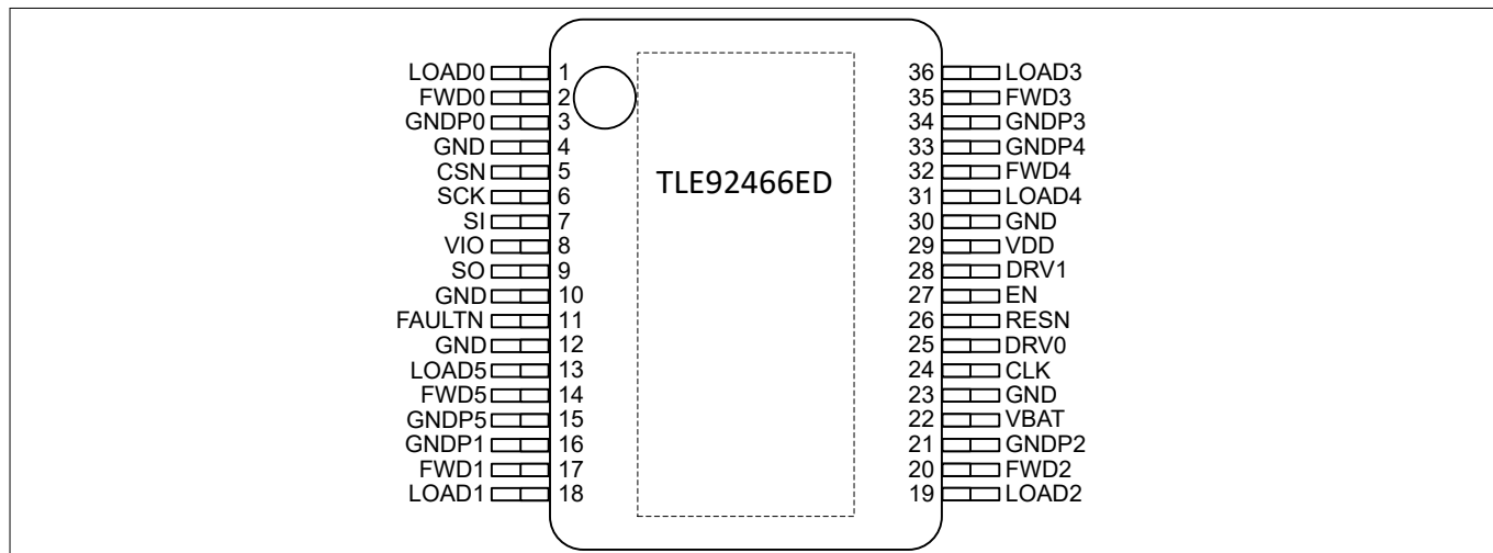
Figure 2 Pin assignment
