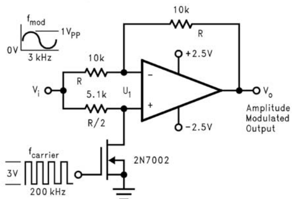
Amplitude Modulator Circuit
