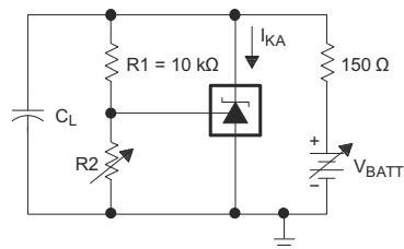
Figure 7-19. Test Circuit for Stability Boundary Conditions
