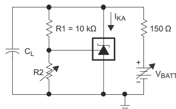
Figure 7-17. Test Circuits for Stability Boundary Conditions
