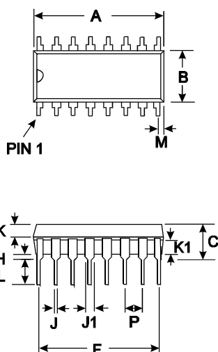
Figure 7 16-pin SOIC (D4) Mechanical Outline: Order as part no. CMX654D4
