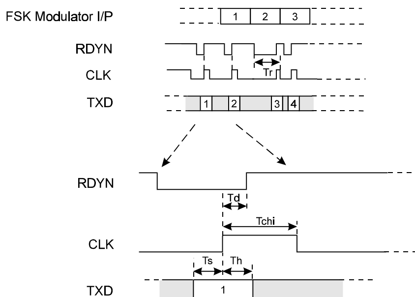
Figure 6 FSK Operation with Tx Data Retiming
