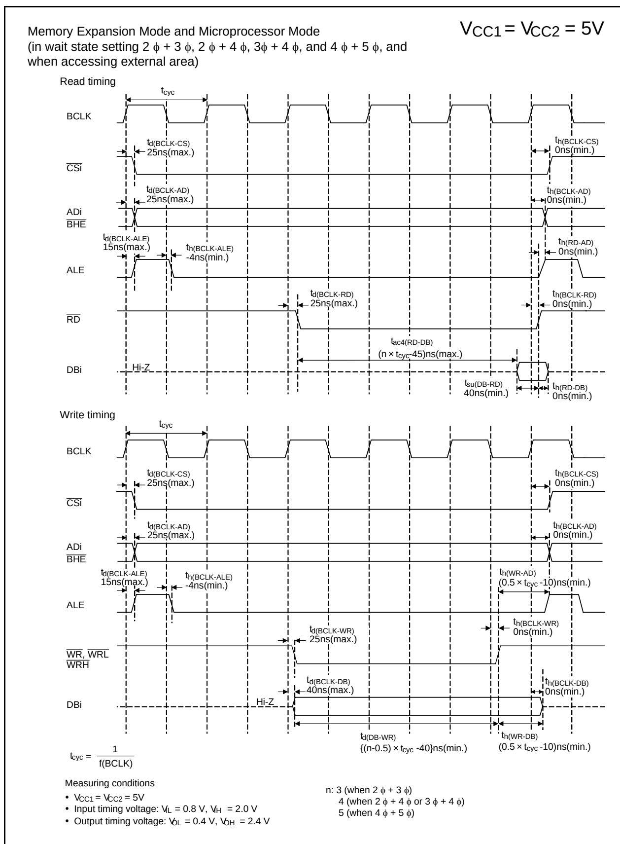
Figure 5.19 Timing Diagram
