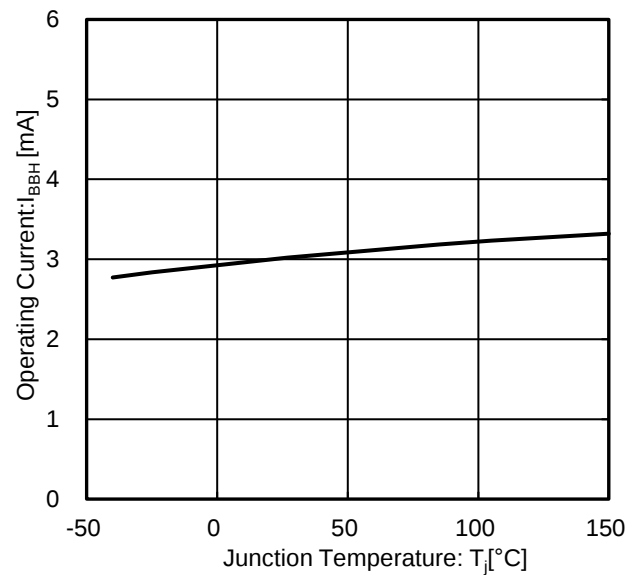
Figure 10. Operating Current vs Junction Temperature
