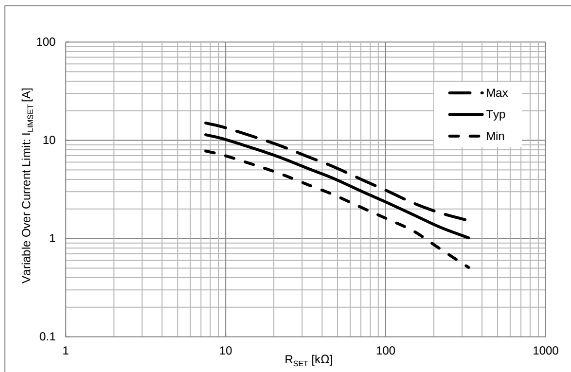
Figure 35. Variable Over Current Limit vs R_{\text{SET}}
