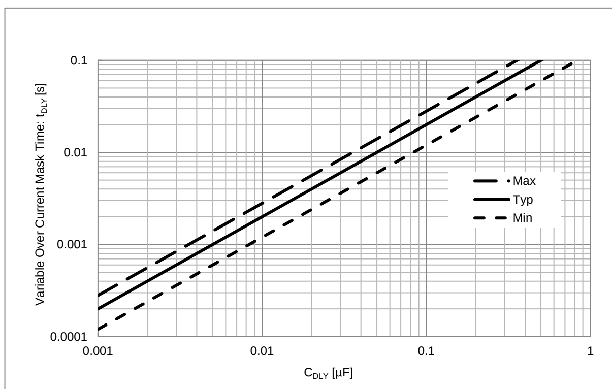
Figure 36. Variable Over Current Mask Time vs C_{DLY}
