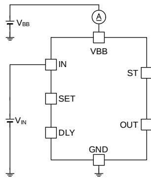
Figure 26. Operating Current
