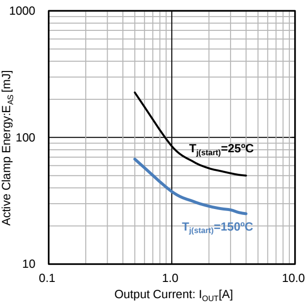
Figure 24. Active Clamp Energy vs Output Current
