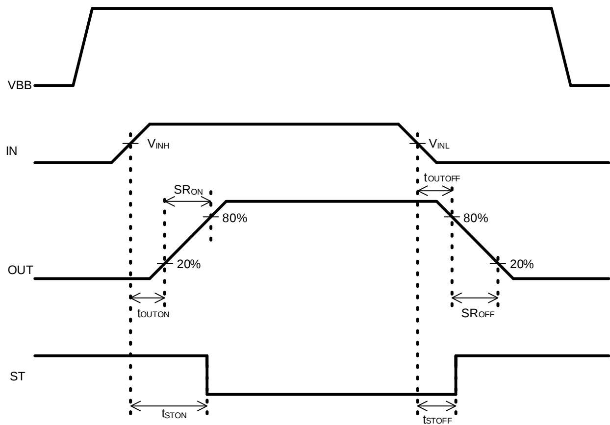
Figure 33. Timing Chart
