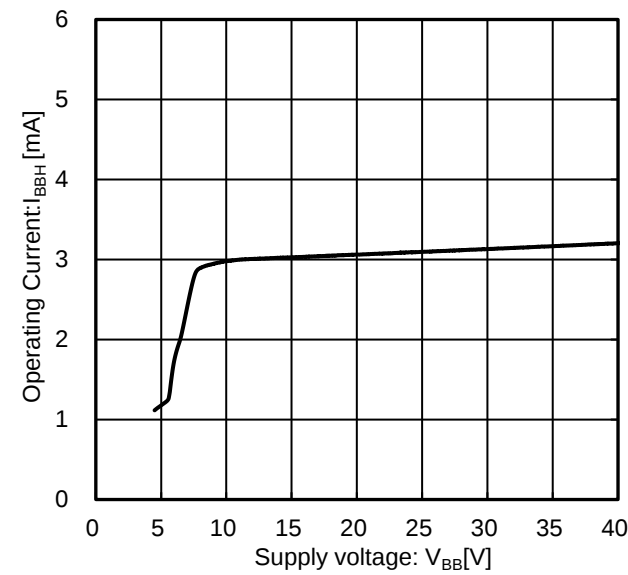
Figure 9. Operating Current vs Supply Voltage
