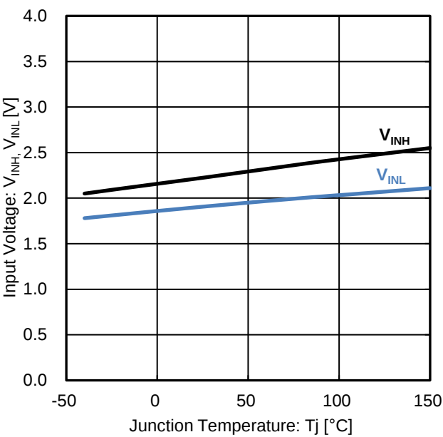
Figure 12. Input Voltage vs Junction Temperature
