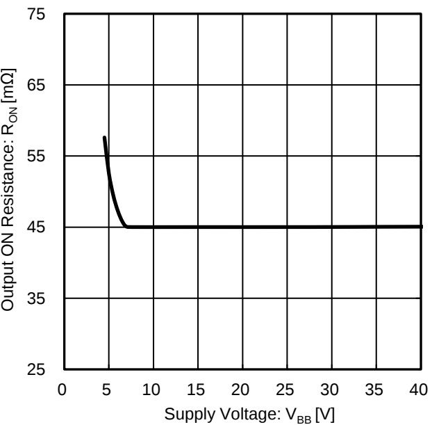
Figure 14. Output ON Resistance vs Supply Voltage
