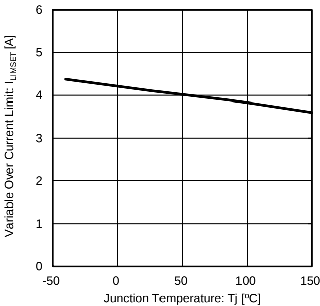
Figure 22. Variable Over Current Limit vs Junction Temperature
