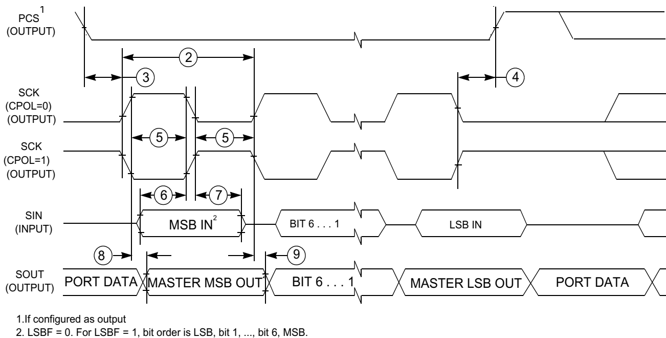
Figure 37. LPSPI Master mode timing (CPHA = 1)
