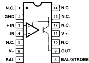
14-PIN HERMETIC DIP (Y-Suffix)
