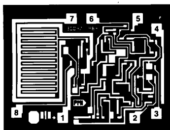
DIE SIZE 0.066 \times 0.050 inch, 3300 sq. mils ( 1.68 \times 1.27 mm, 2.13 sq. mm)
