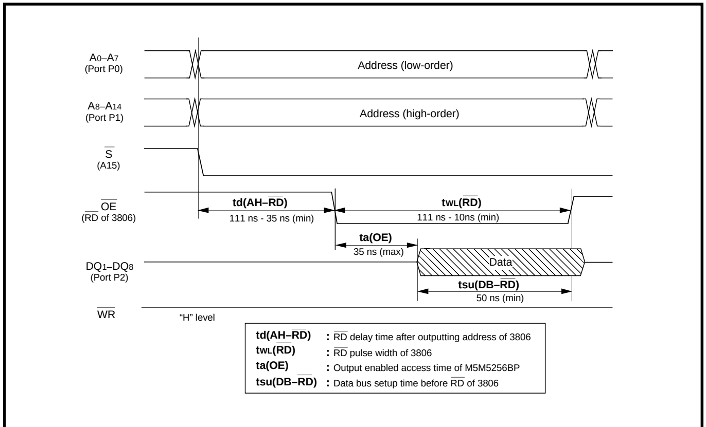
Fig. 2.5.9 Read-cycle (OE access, SRAM) [High-speed version]
