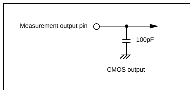
Fig. 3.1.1 Circuit for measuring output switching characteristics (1)
