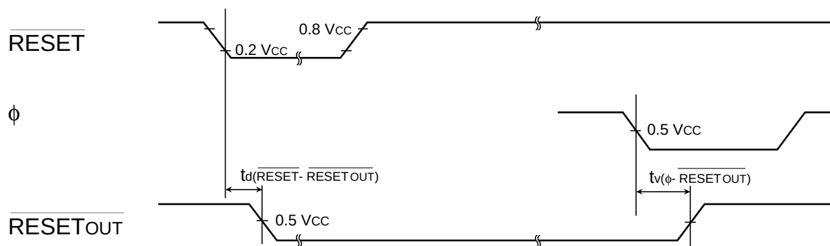
Fig. 3.1.4 Timing diagram (in memory expansion mode and microprocessor mode) (1)
