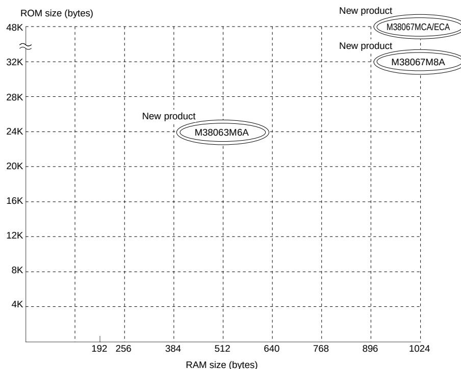
Fig. 7 Memory expansion plan (High-speed version)
