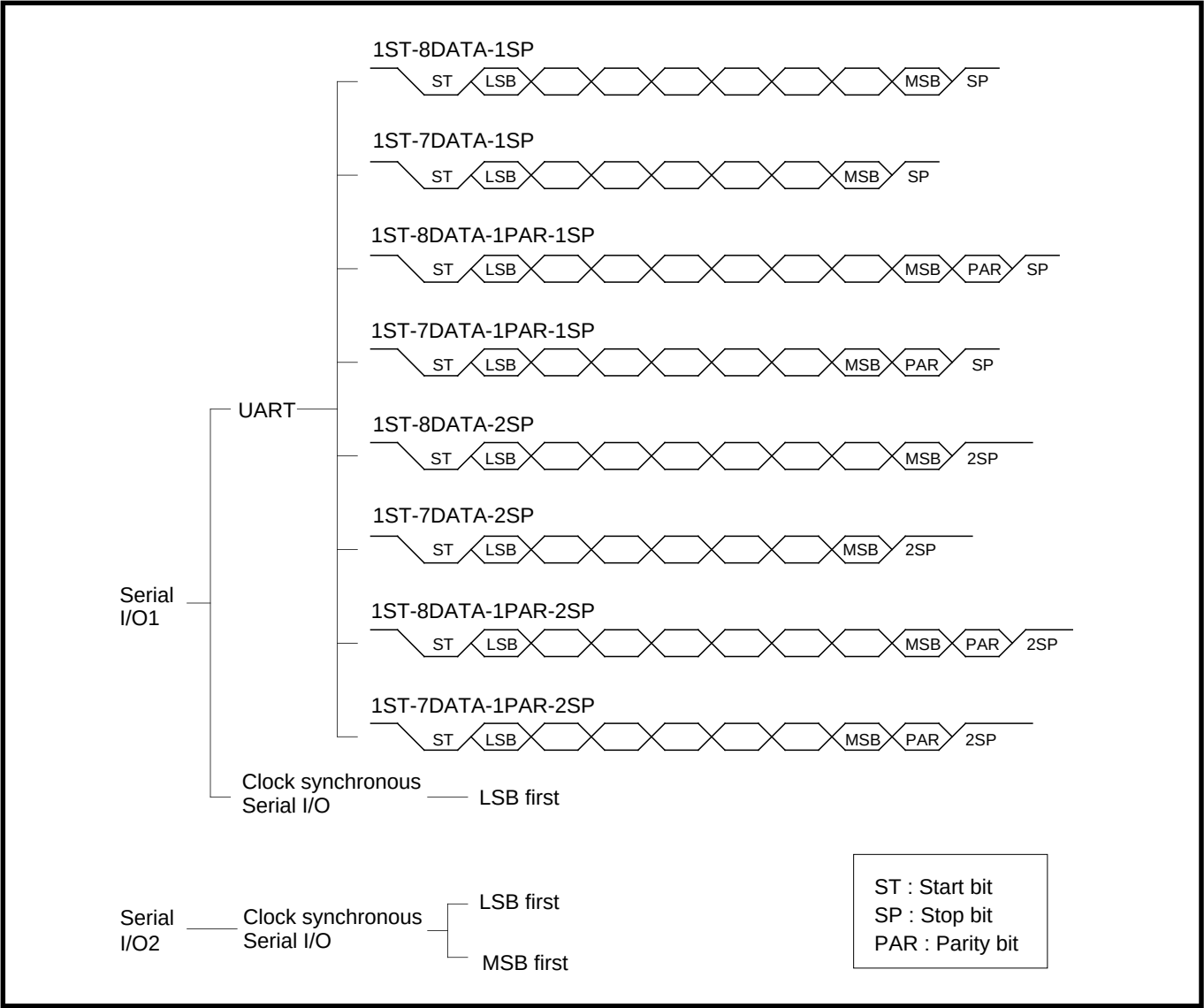
Fig. 2.3.16 Setting of Serial I/O transfer data format
