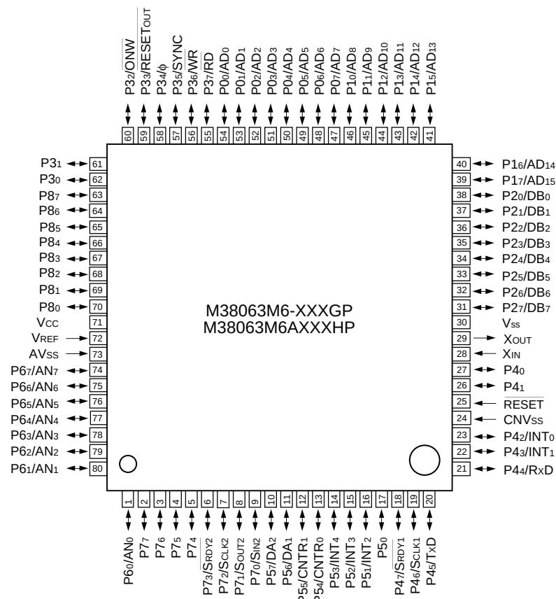
Package type : 80P6S-A/80P6D-A 80-pin plastic-molded QFP
