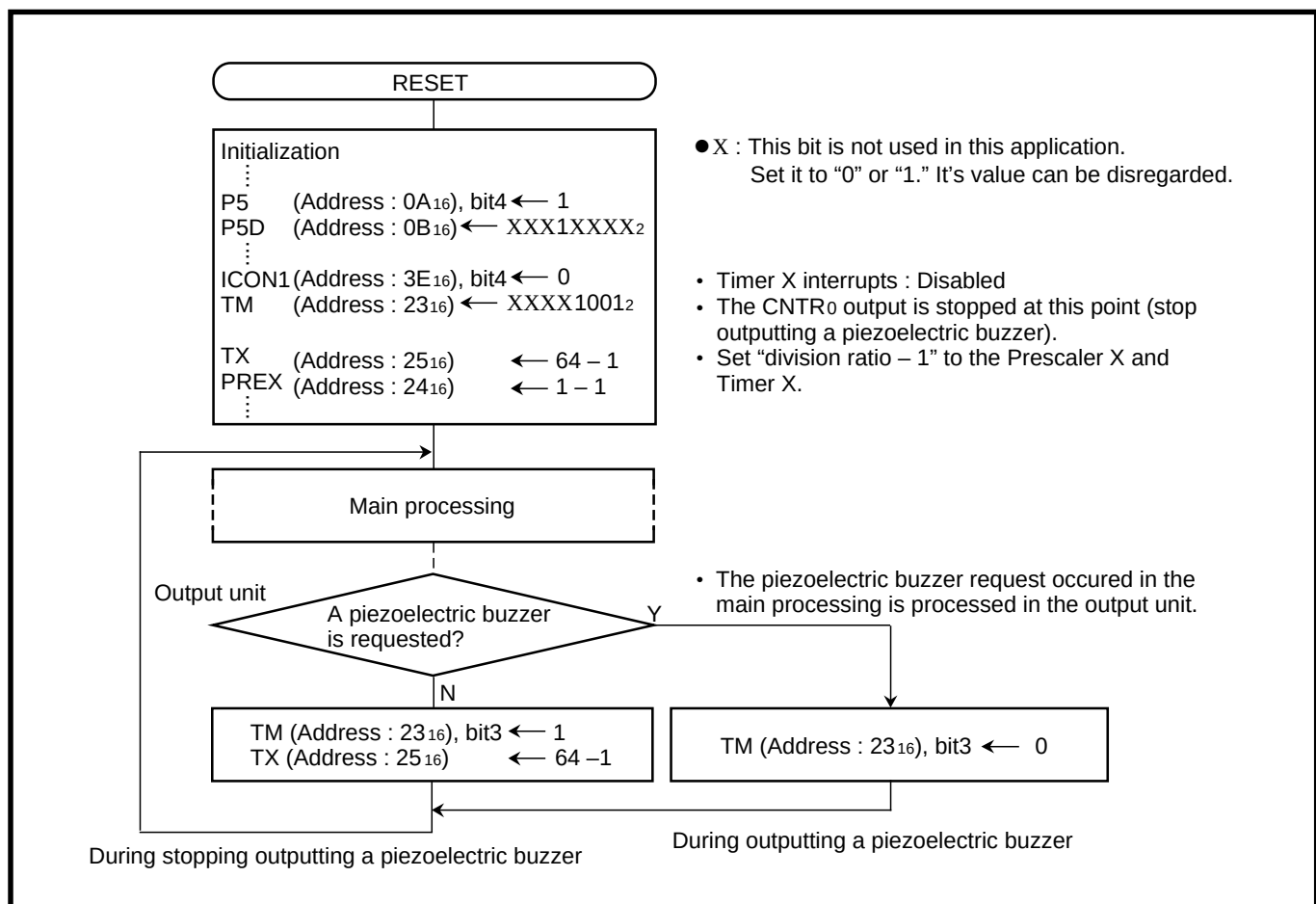
Fig. 2.2.16 Control procedure [Piezoelectric buzzer output]
