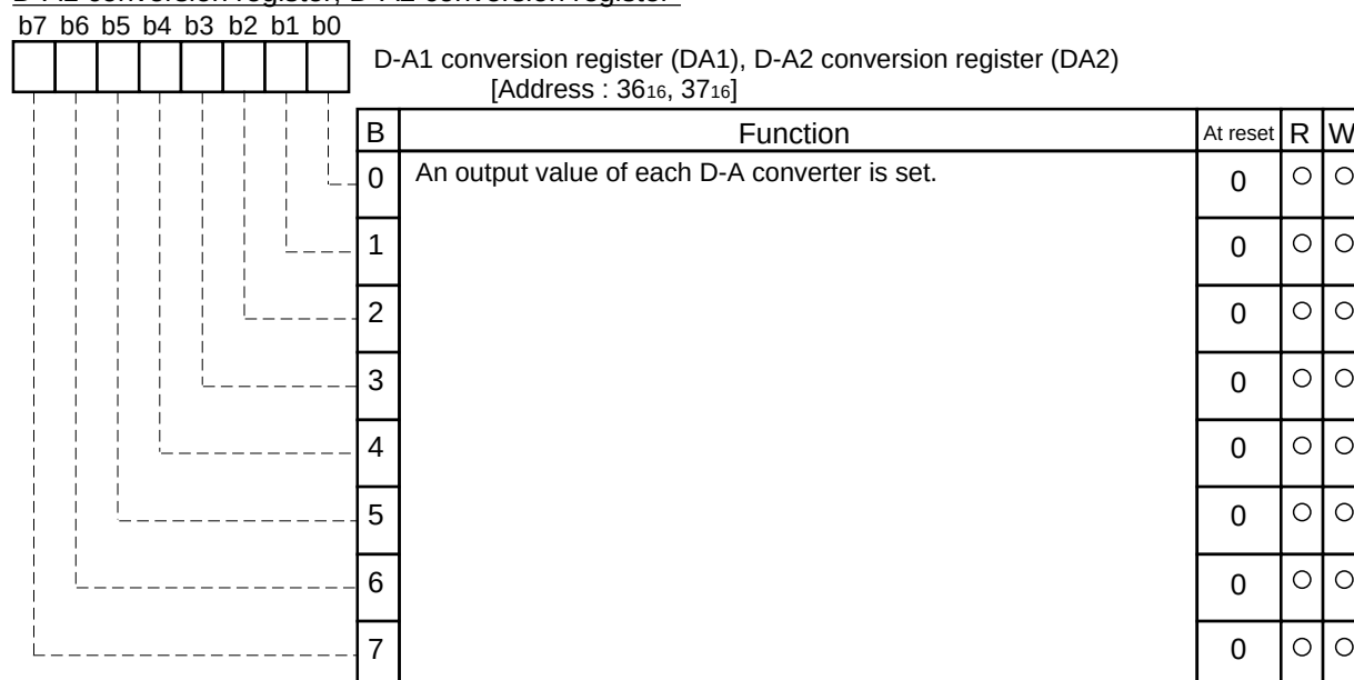
D-A1 conversion register, D-A2 conversion register
