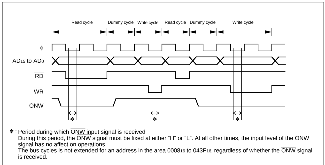
Fig. 39 \overline{\text{ONW}} function timing
