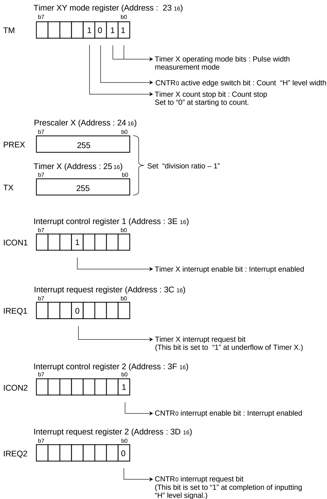
Fig. 2.2.21 Setting of related registers [Measurement of pulse width]
