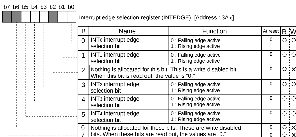
Interrupt edge selection register
