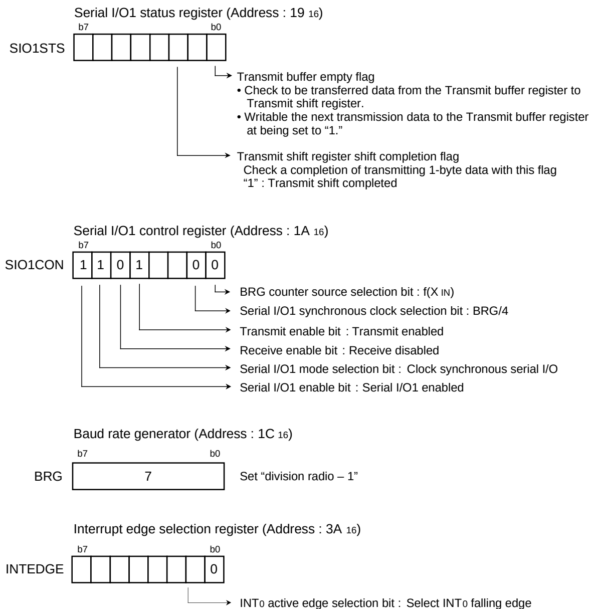
Fig. 2.3.19 Setting of related registers at a transmitting side [Communication using a clock synchronous serial I/O]
