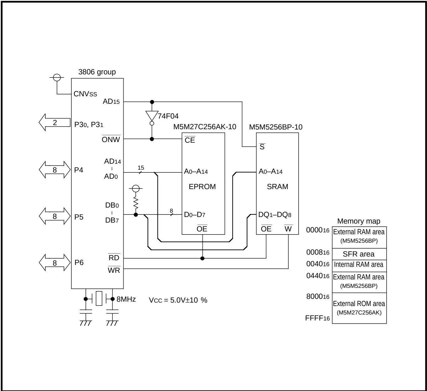
Fig. 2.5.7 Application example of the \overline{\text{ONW}} function
