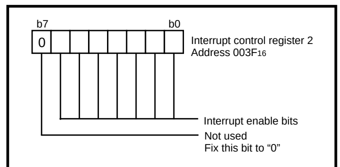
Fig. 3.3.1 Structure of interrupt control register 2
