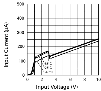
Input Current v Input Voltage
