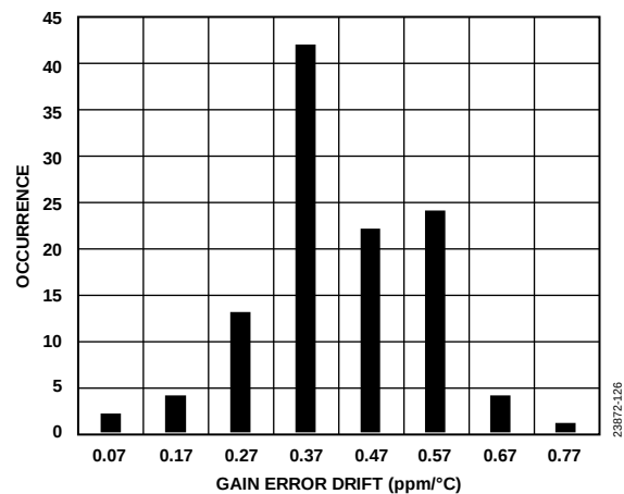
Figure 19. Gain Error Drift Distribution Histogram
