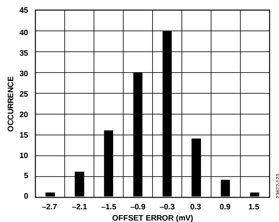
Figure 16. Offset Error Distribution Histogram
