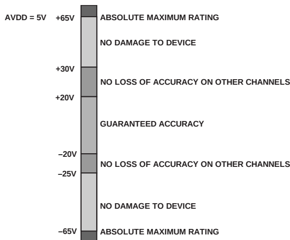
Figure 28. Absolute Input Pin Voltages, AVDD = 5 V
