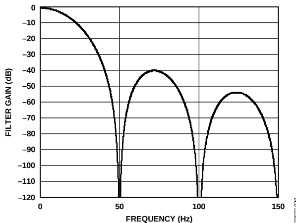
Figure 33. Sinc3 Filter Response
