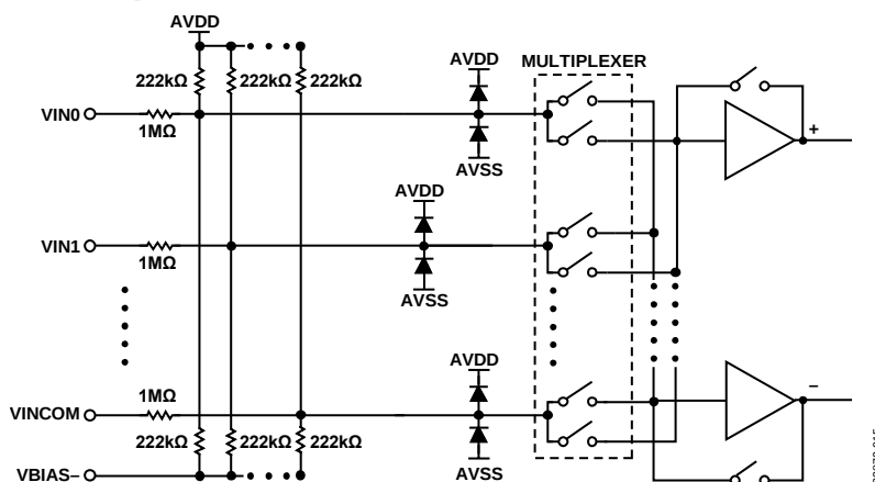
Figure 26. Simplified Voltage Input Circuits
