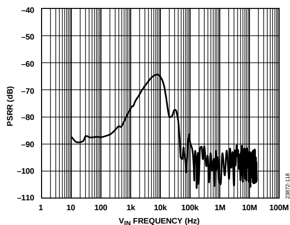
Figure 15. PSRR vs. V_{IN} Frequency
