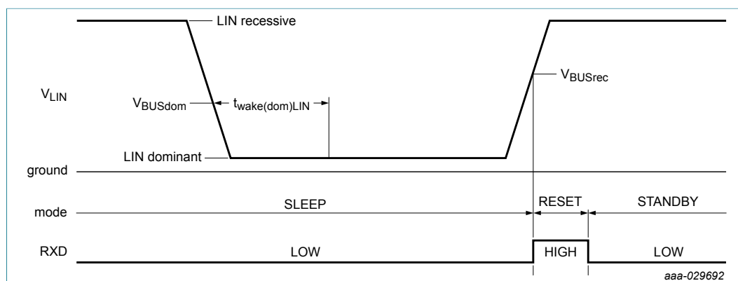
Figure 8. Principle of remote wake-up via LIN bus during SLEEP mode
