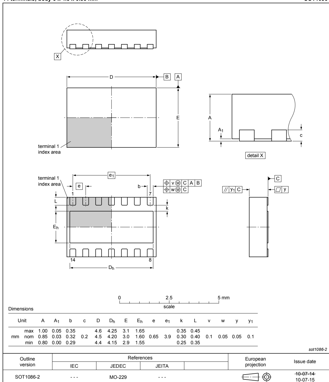
Figure 14. Package outline
