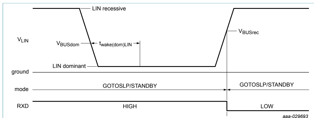
Figure 9. Principle of remote wake-up via LIN bus during GOTOSLP and STANDBY mode
