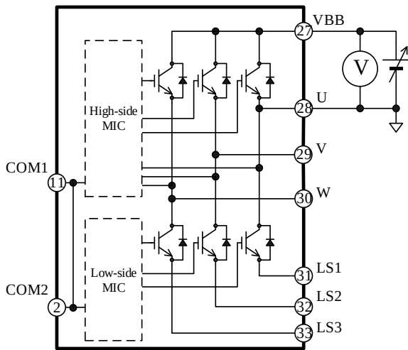
Figure 13-3. Typical Measurement Circuit for High-side Transistor ( Q_{1H} ) in U-phase
