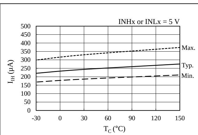
Figure 15-13. Input Current at High Level ( I_{IH} or I_{IL} ), I_{IH} vs. T_C
