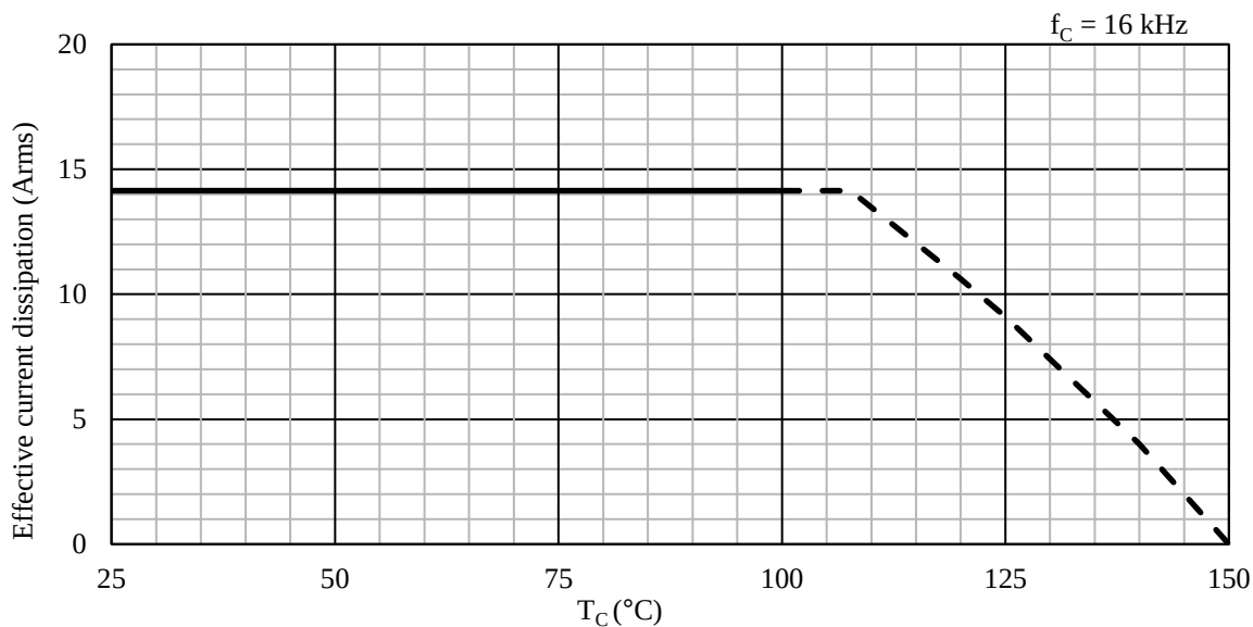
Figure 15-35. Allowable Effective Current ( f_C = 16 kHz)
