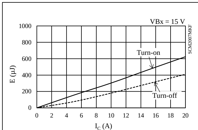
Figure 15-32. High-side Switching Loss ( T_J = 125^\circ\text{C} )
