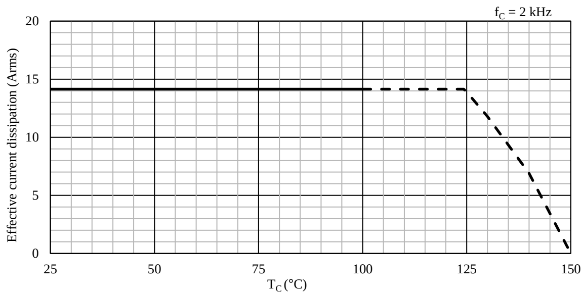
Figure 15-34. Allowable Effective Current ( f_C = 2 kHz)
