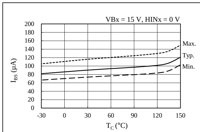
Figure 15-4. Logic Supply Current in 1-phase Operation ( HINx = 0\text{ V} ), I_{BS} vs. T_C
