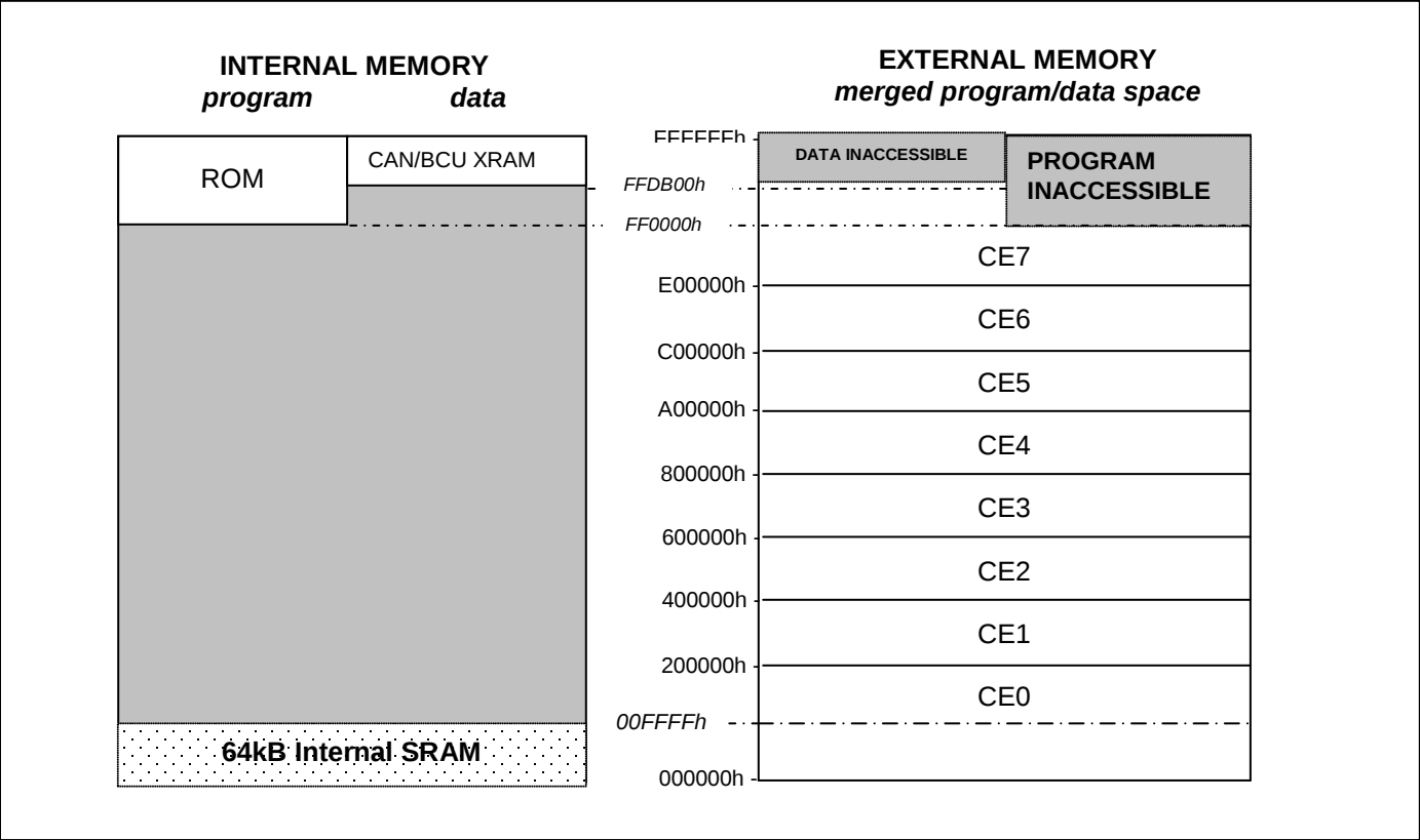
Figure 14. Memory Map Following Execution of ROM_Init on DS80C410/DS80C411
