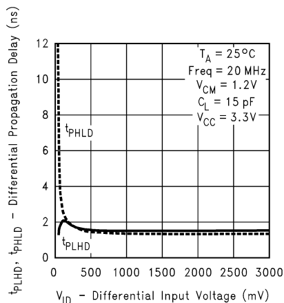
Differential Propagation Delay vs Differential Input Voltage
