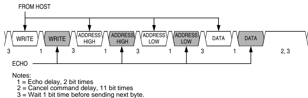
Figure 19-16. Write Transaction
