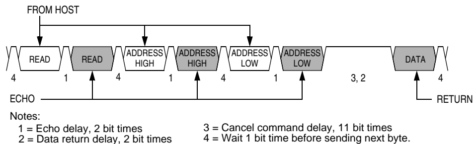
Figure 19-15. Read Transaction
