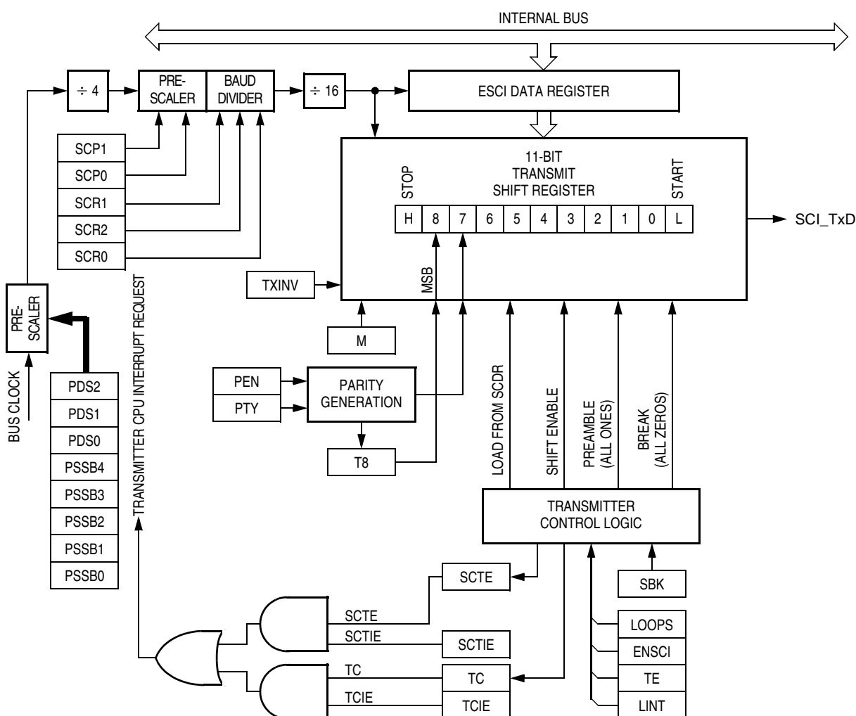
Figure 14-5. ESCI Transmitter
