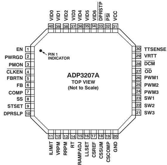
Figure 5. Pin Configuration
