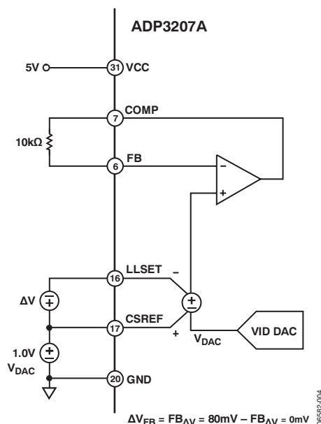
Figure 4. Positioning Accuracy
