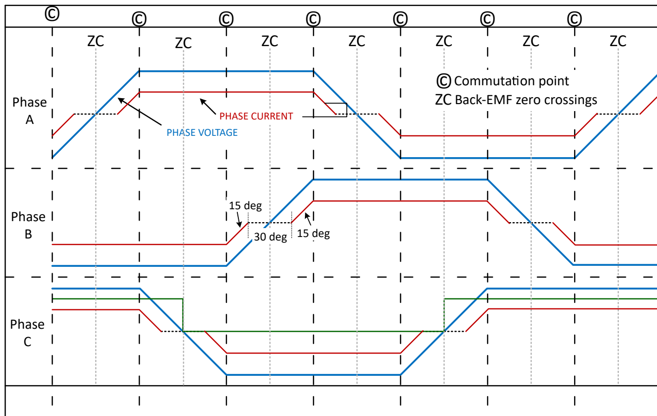
Figure 8-29. 150° commutation
