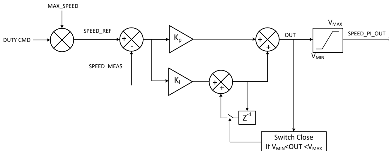
Figure 8-32. Speed Loop
