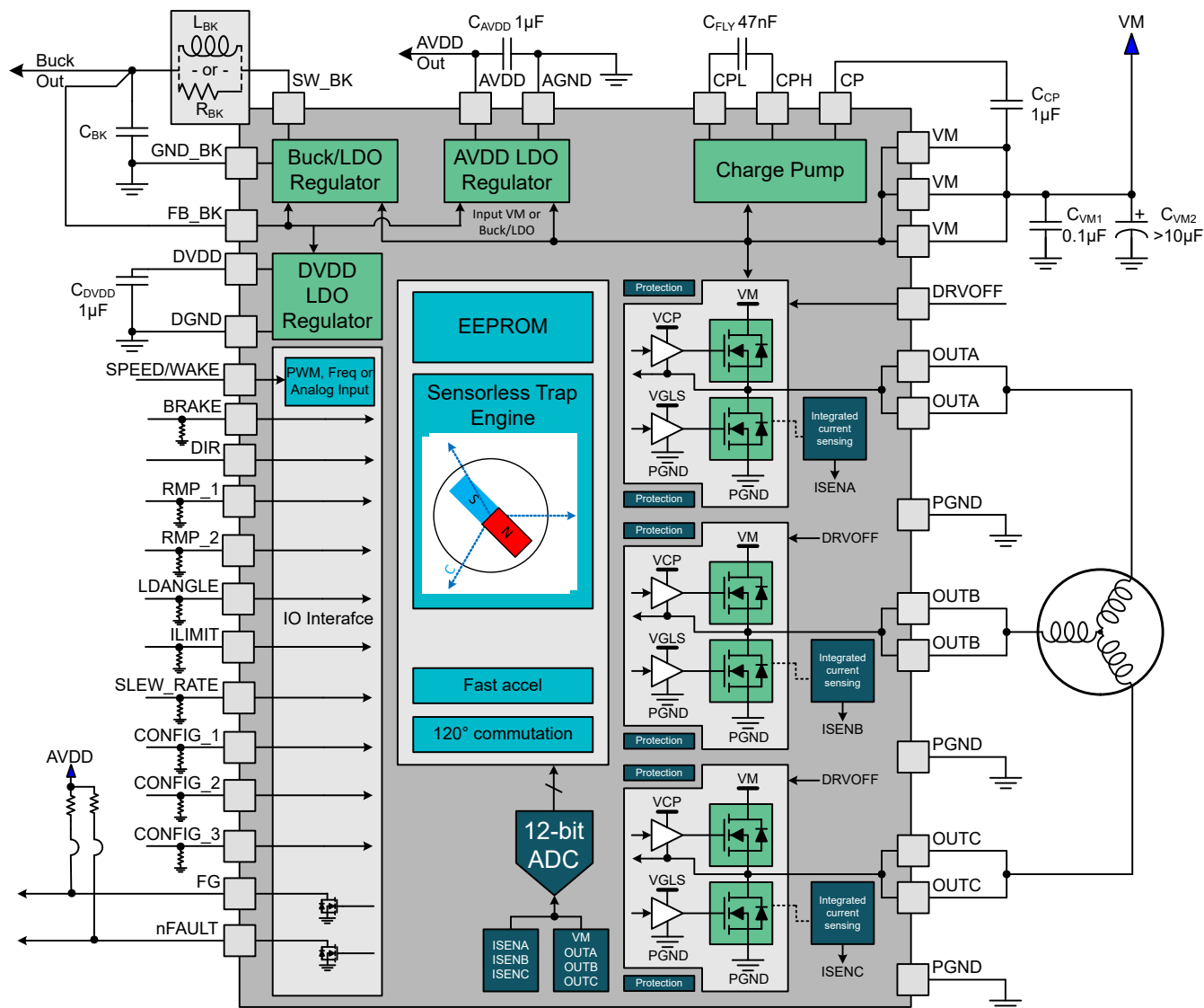
Figure 8-2. MCT8316AT Functional Block Diagram
