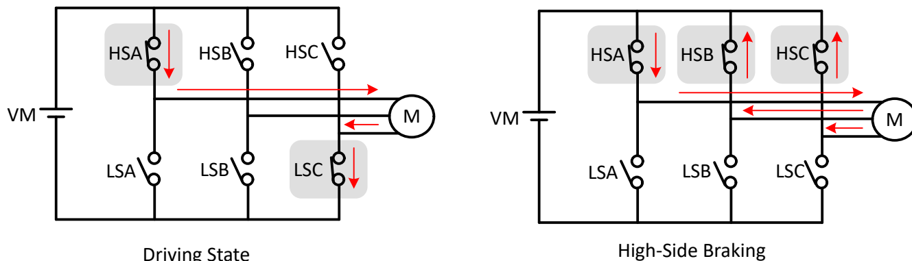
Figure 8-44. High-Side Braking
