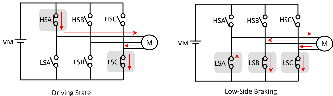
Figure 8-43. Low-Side Braking
