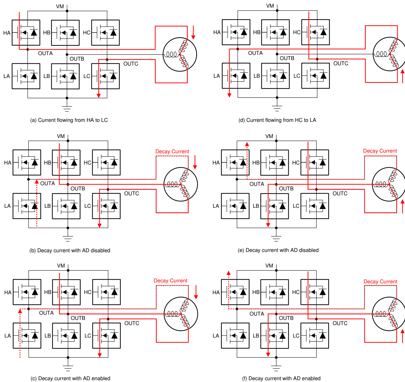
Figure 8-38. Active Demagnetization in BLDC Motor Commutation
