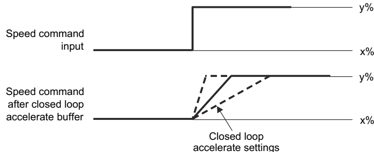
Figure 8-31. Closed loop accelerate
