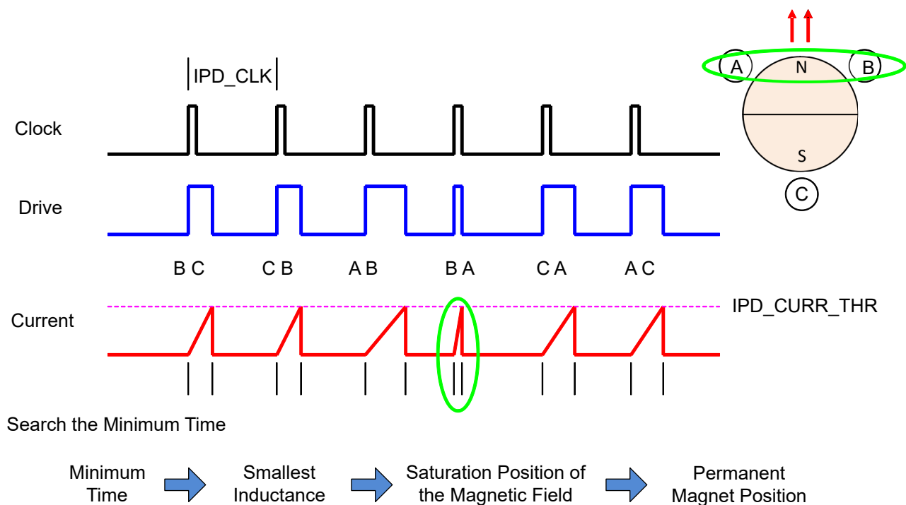
Figure 8-21. IPD Function
