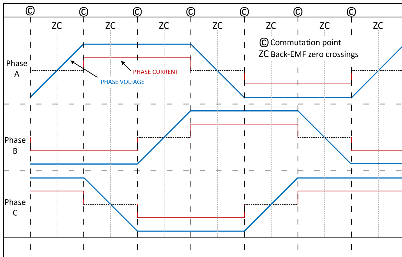
Figure 8-25. 120° commutation
