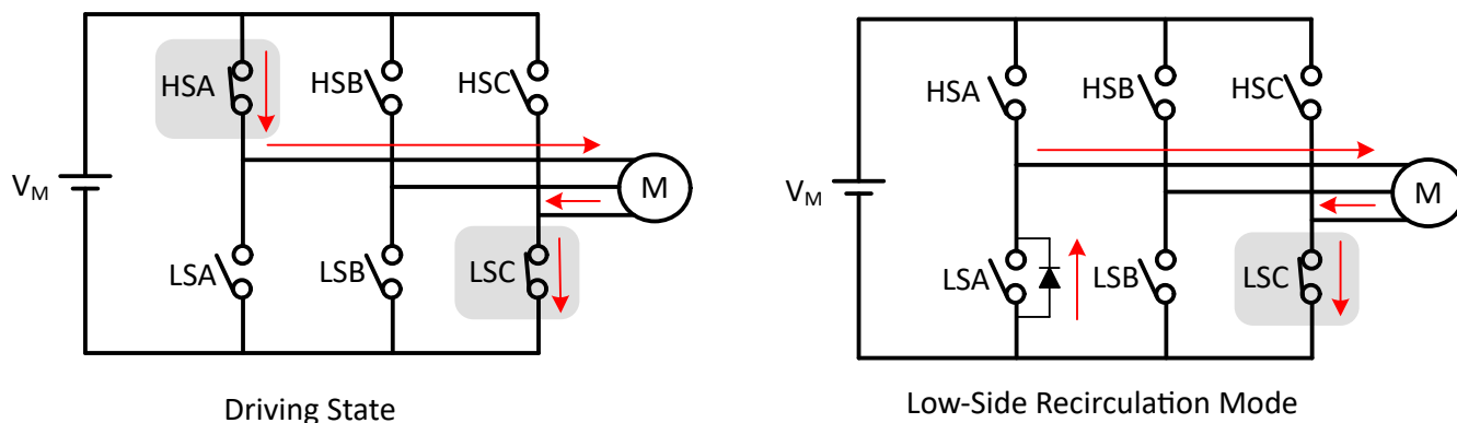
Figure 8-41. Low-Side Recirculation
