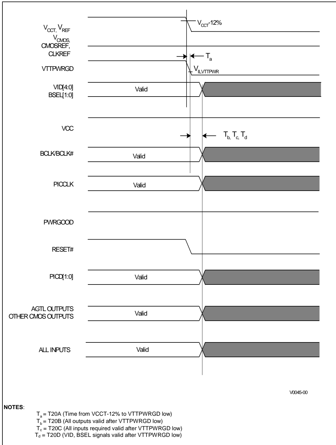
Figure 14. Power Down Sequencing and Timings (V CCT Leading)
