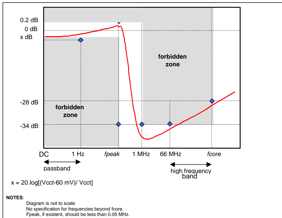
Figure 30. PLL Filter Specifications
