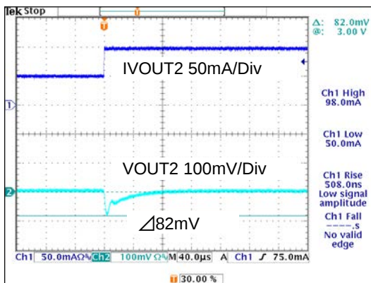
Figure 31. Load Response(Rise) (VBAT=3.6V, Cout=4.7 \mu F, Ta=25°C, Iout=50mA→100mA, Tr=0.5 \mu s)
