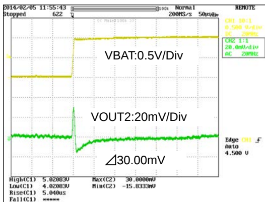
Figure 23. VBAT Response(Rise) (VBAT=4V→5V, Cout=4.7 \mu F, Ta=25°C, Tf=0.5 \mu s)
