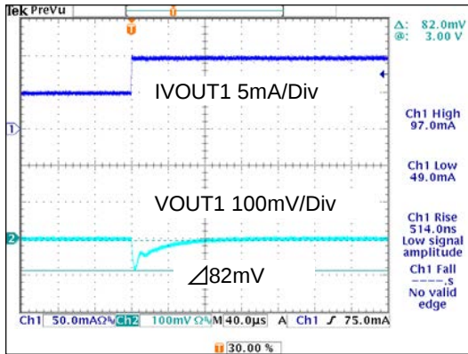
Figure 29. Load Response(Rise) (VBAT=3.6V, Cout=4.7 \mu F, Ta=25°C, F, Iout=50mA→100mA, Tr=0.5 \mu s)
