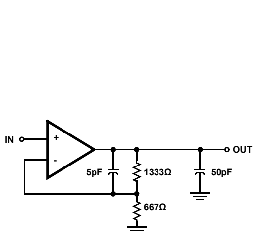
FIGURE 1. SLEW RATE AND SETTLING TIME
