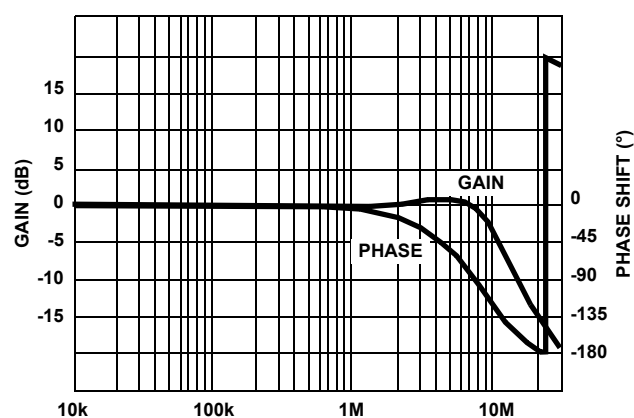
FIGURE 7. FREQUENCY RESPONSE FOR INVERTING UNITY GAIN CIRCUIT
