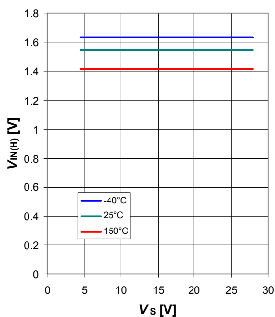
Figure 42 HIGH Level Input Voltage V_{IN(H)} = f(V_S, T_J)
