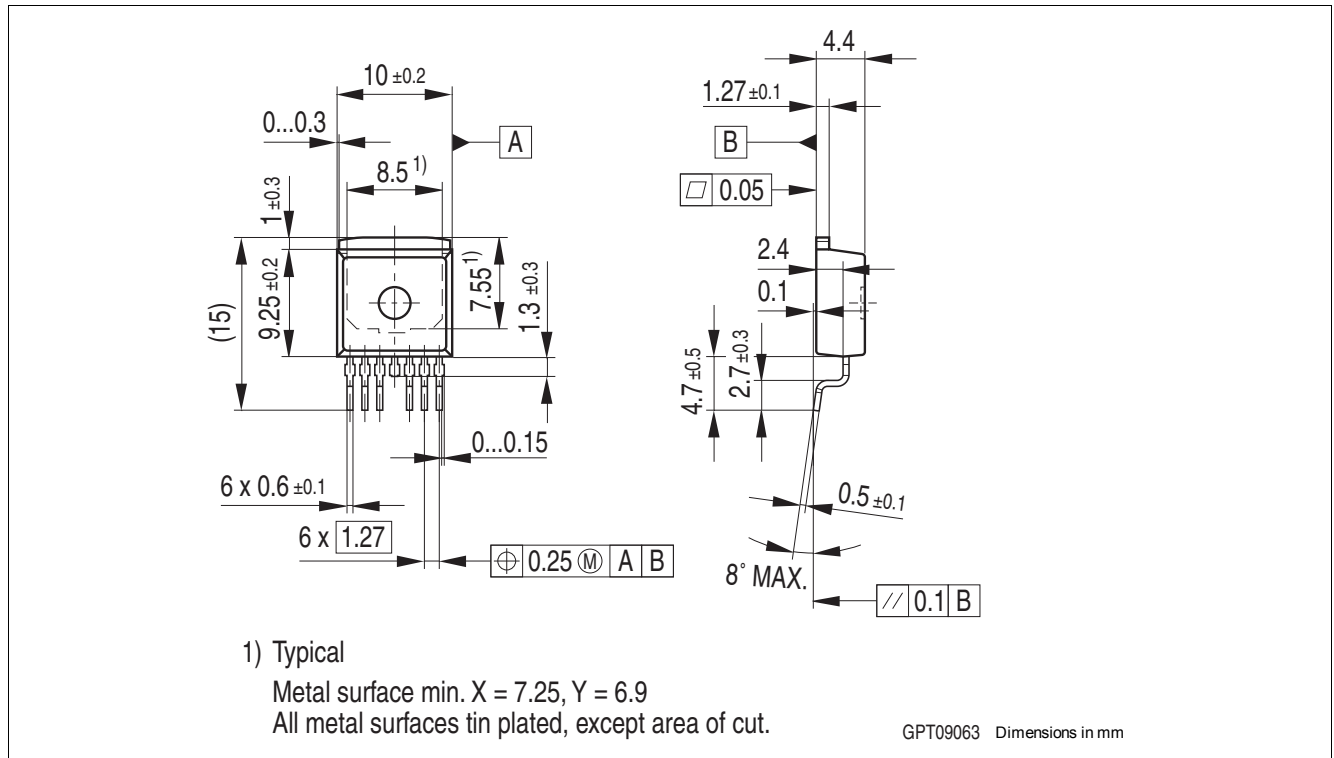
Figure 50 PG-TO-263-7-8 (RoHS-Compliant)
