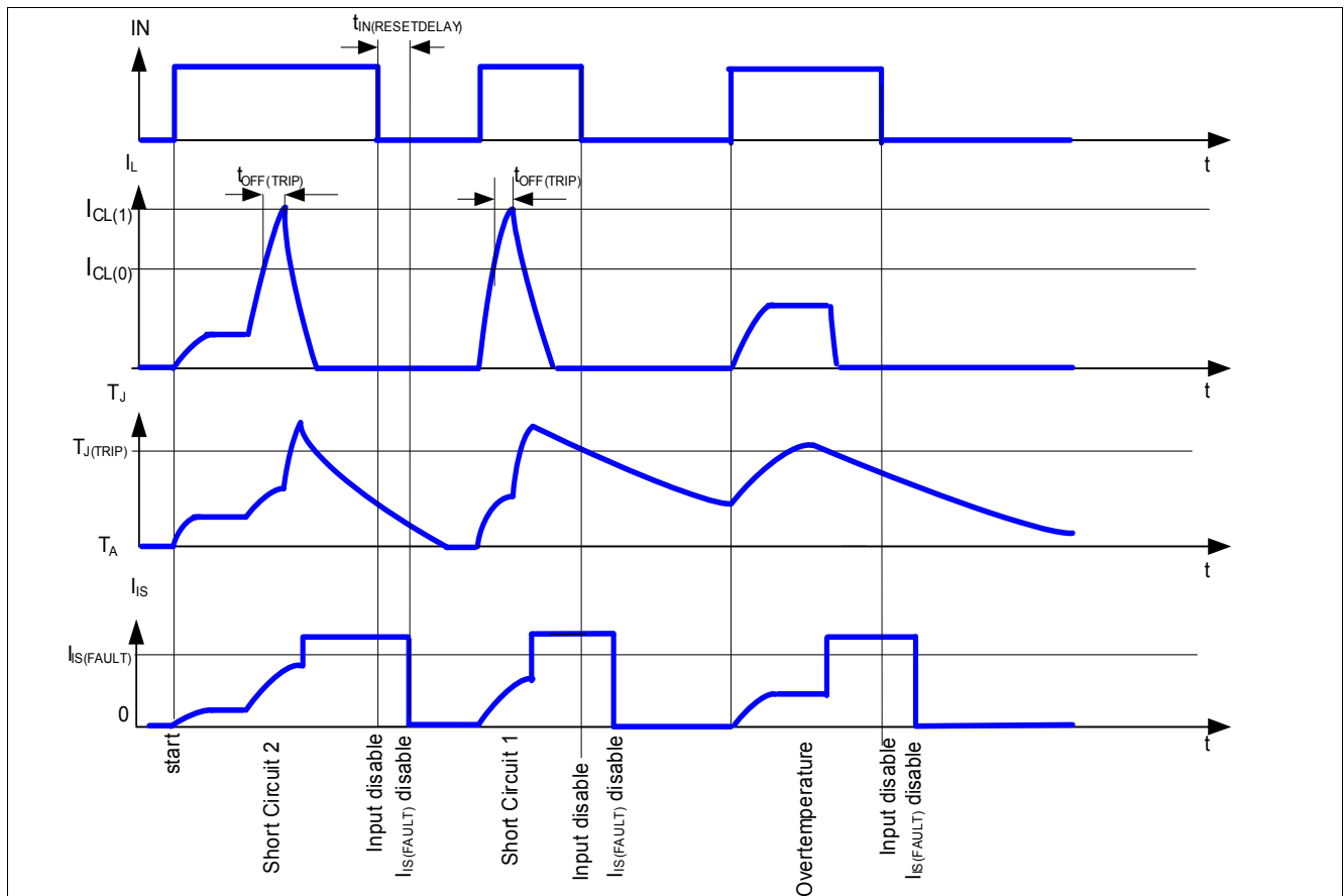
Figure 22 Overload Protection
