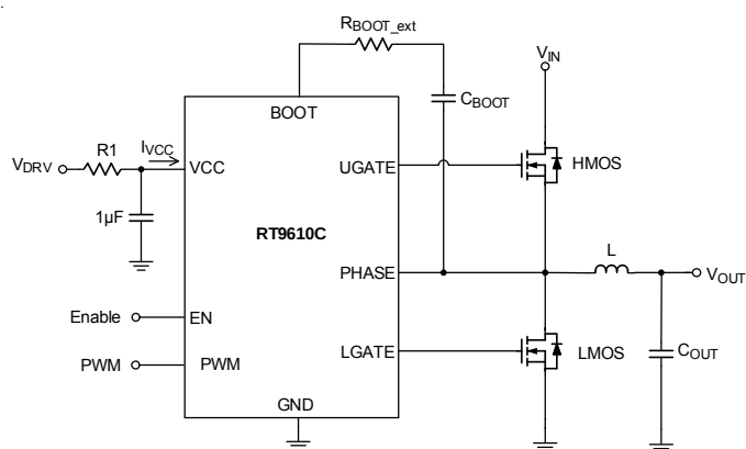
Figure 2. Part of Bootstrap Circuit of RT9610C
