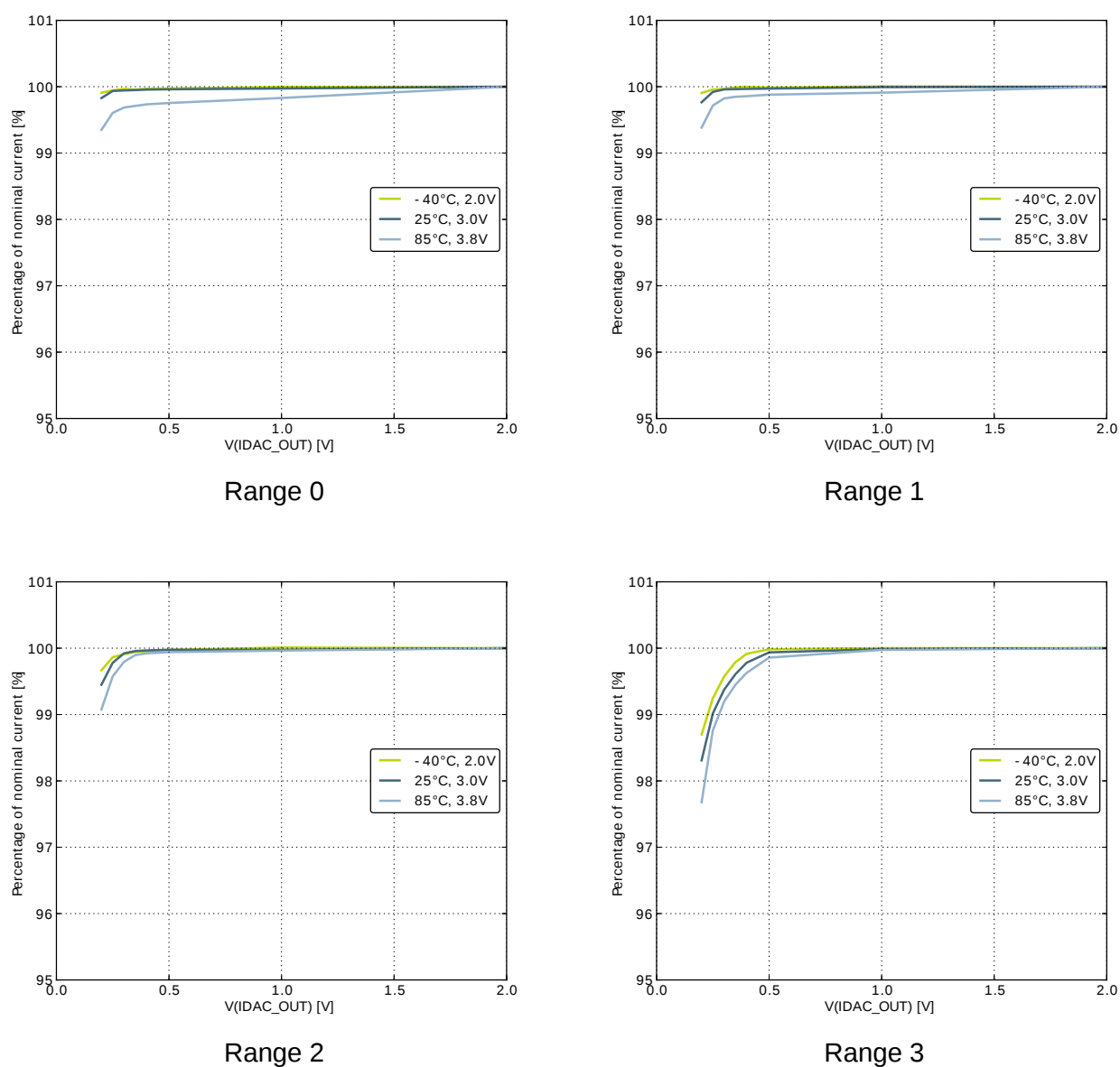
Figure 3.37. IDAC linearity
